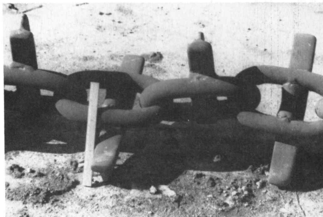
Ely chain link.
