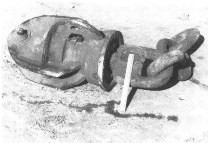
Swivel made from crawler tractor track roller.
