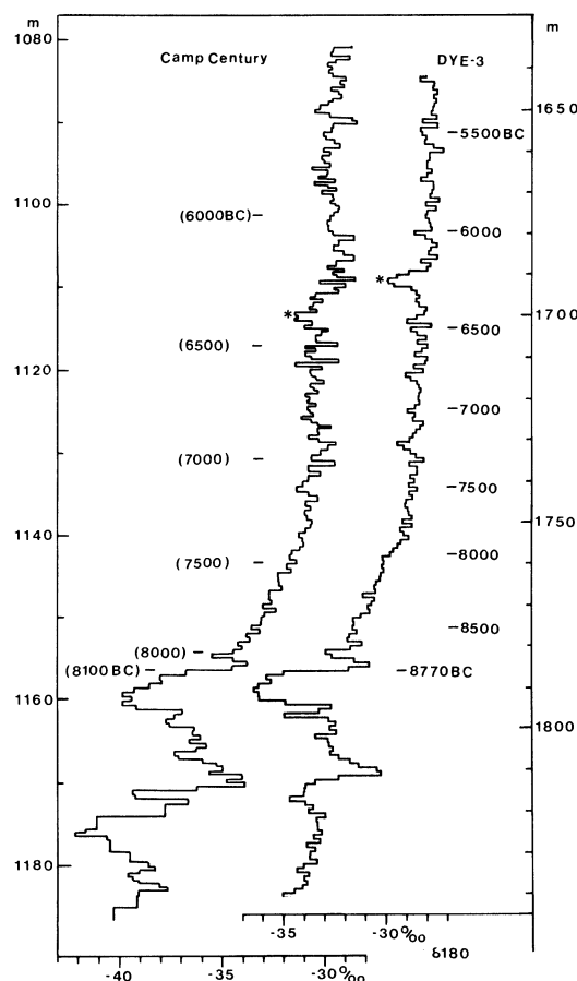
Fig 3. Comparison between dates and \delta^{18}\text{O} profiles of the Camp Century core (Hammer et al. , 1978) and the Dye 3 core. The YD/PB boundary and the strong \delta oscillations (*) in the two cores are supposed to be simultaneous. The ages (in brackets) for the lower part of the Camp Century core therefore need considerable correction in order to agree with the more accurate dates of the Dye 3 core.
