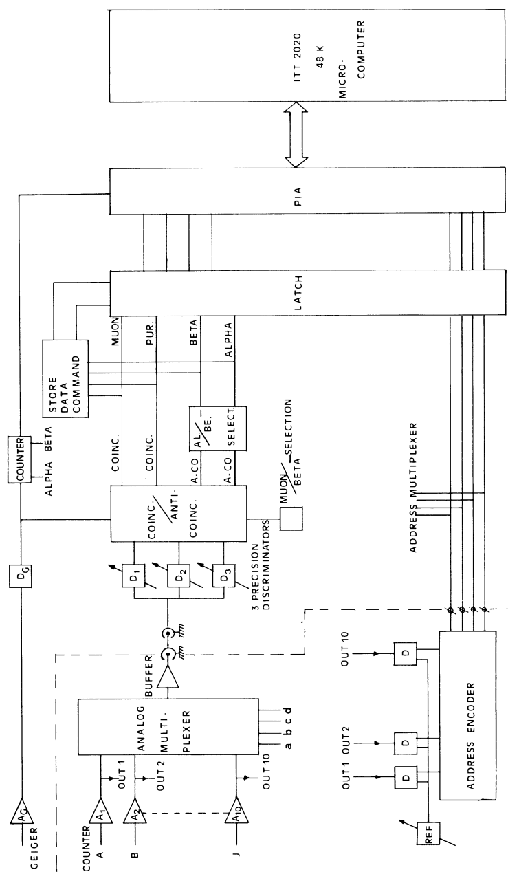
Fig 2. Data-acquisition system
