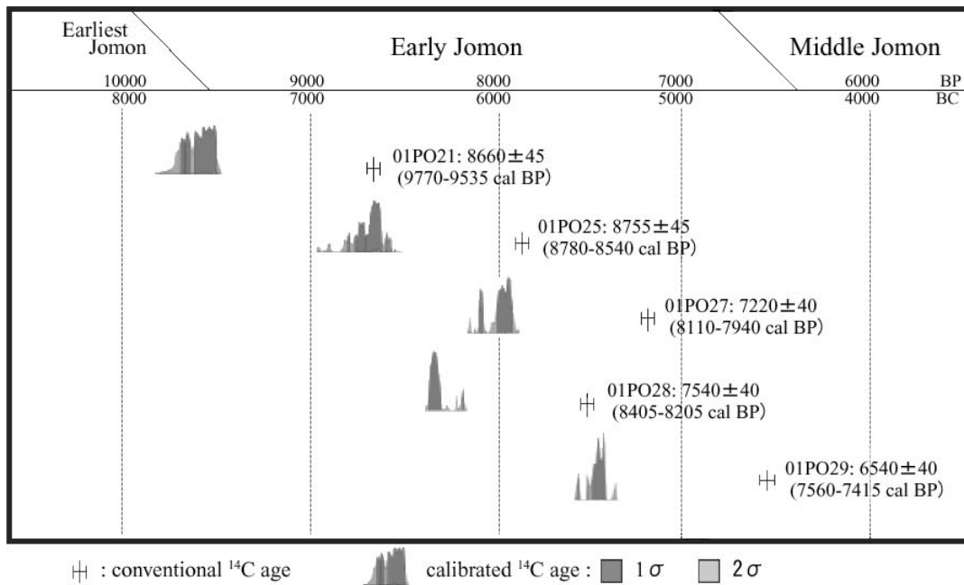
Figure 4 ^{14}\text{C} ages for fiber pottery in Myouonji Cave site, Japan, during the Jomon period
