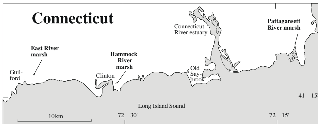
Figure 1 Location of the three study sites
