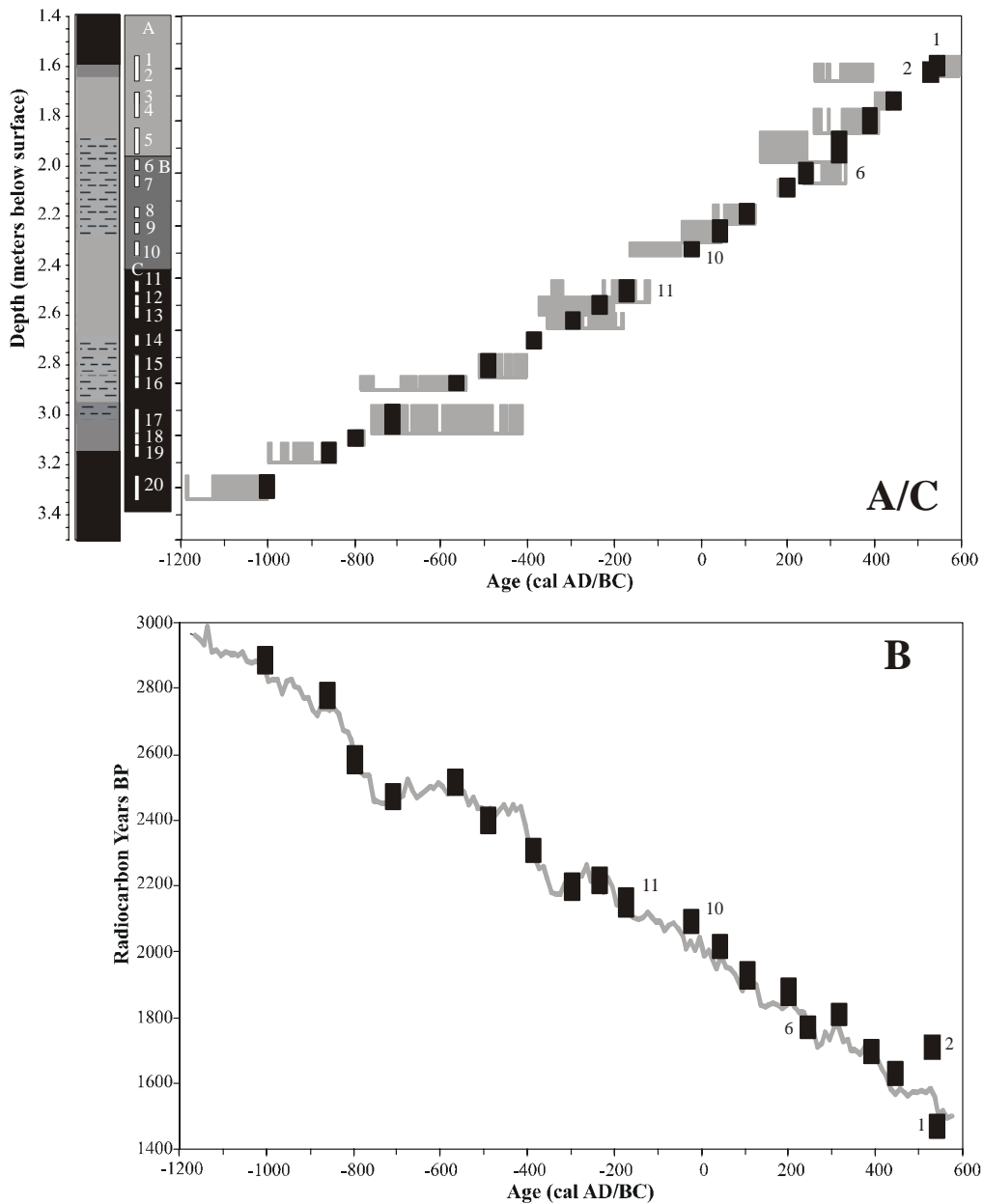
Figure 3 Hammock River marsh. A. Stratigraphic column and accompanying, individually calibrated, AMS ^{14}\text{C} dates (grey error boxes); B. Wiggle-matched dates plotted against the ^{14}\text{C} calibration curve; C. Wiggle-matched sub-groups (second column on left) and wiggle-matched dates (black error boxes); Dates 11 and 6 are “tie dates” between sub-groups.
