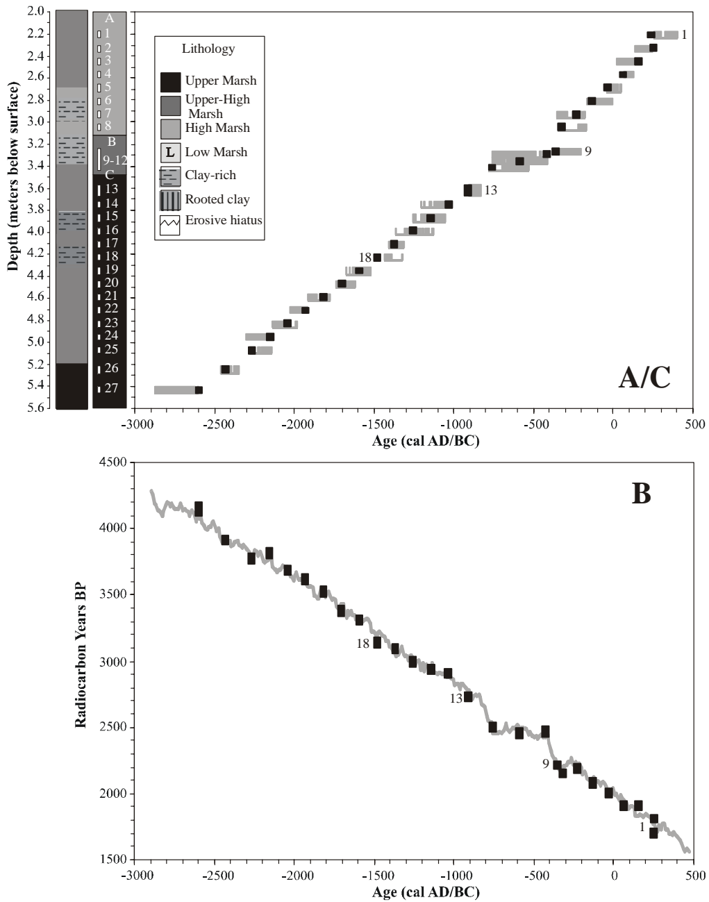
Figure 2 Pattagansett River marsh. A. Stratigraphic column and accompanying, individually calibrated, AMS ^{14}\text{C} dates (grey error boxes); B. Wiggle-matched dates plotted against the ^{14}\text{C} calibration curve; C. Wiggle-matched sub-groups (second column on left) and wiggle-matched dates (black error boxes); Dates 13 and 9 are "tie dates" between sub-groups.
