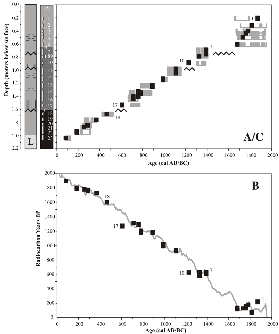
Figure 4 East River marsh. A. Stratigraphic column and accompanying, individually calibrated AMS ^{14}\text{C} dates (grey error boxes); B. Wiggle-matched dates plotted against the ^{14}\text{C} calibration curve; C. Wiggle-matched subgroups (second column on left) and wiggle-matched dates (black error boxes).
