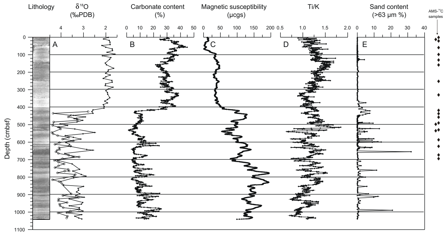
Figure 3 Sediment composition in core DS97-2P: A) \delta^{18}\text{O} of planktonic foraminifera G. bulloides (●) and N. pachyderma (sinistral) (○), B) carbonate content, C) magnetic susceptibility, D) Ti/K ratio, E) sand content (>63 μm) in terrigenous sediment fraction. The digital image on the left illustrates the variations in lithology.
