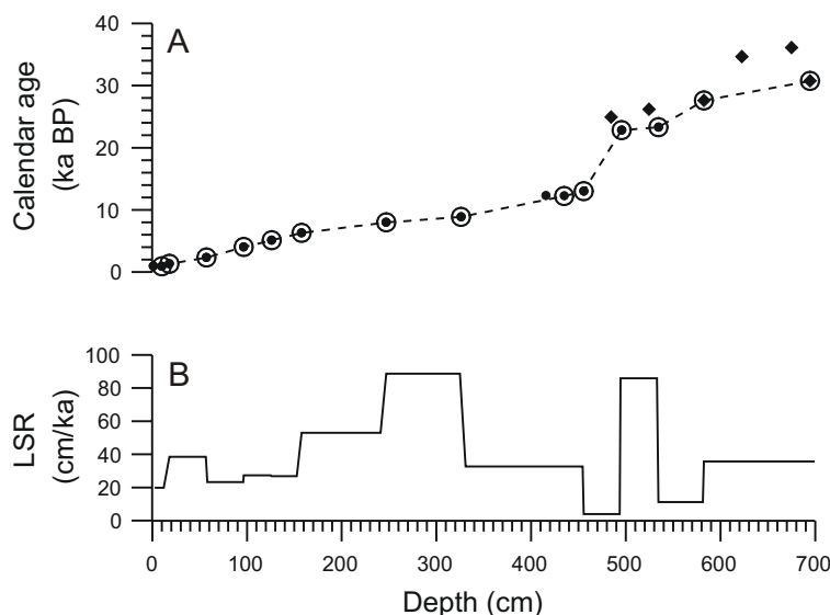
Figure 2 Age model of core DS97-2P: A) Calendar age-depth profile of AMS- 14 C dated samples. 14 C ages were calibrated according to (●) the Calib 4.2 program (Stuiver and Reimer 1993) or (◐) the regression equation which describes the relationship between 14 C and Th/U ages (E Bard, 4th International Congress on Paleoceanography, Kiel, 1992). Encircled symbols indicate the samples that were used to construct the age model. Data are listed in Table 1. B) Linear-sedimentation rate (LSR).
