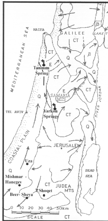
Figure 1 The conceptual flow model of the Yarkon-Taninim aquifer as proposed by Mandel (1961) and Baida et al. (1970). The model would have water from the Beer-sheva region flow north to drain at the Yarkon and Taninim springs. The position of the wells in Table 3 are shown.
