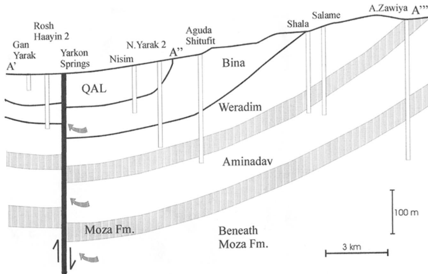
Figure 3 Hydrogeological section showing the different hydrological units that are exploited by the water wells in the study area. The accepted hydrologic conceptual model does not consider that the Judea Group aquifer is divided into independent aquifer units. It is the deeper formations that have been found by present study to be the major contributors to the Yarkon Springs. They are significantly younger, cooler, and contain lower salt contents than the water in the upper aquifer. It is the latter that has been, until now, considered to represent the Judea Group (Yarkon-Taninim) aquifer.
