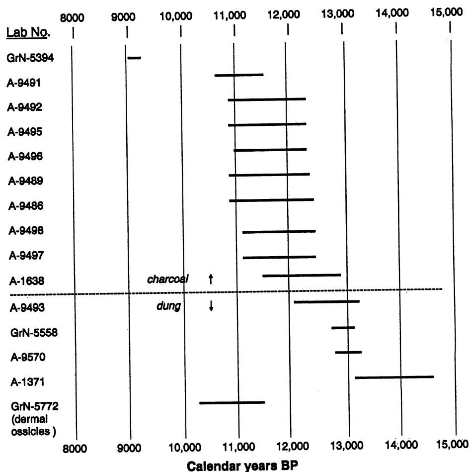
Fig. 4B. Dates with standard deviations 200 yr, calibrated using curve of Huguen et al. (1998)
