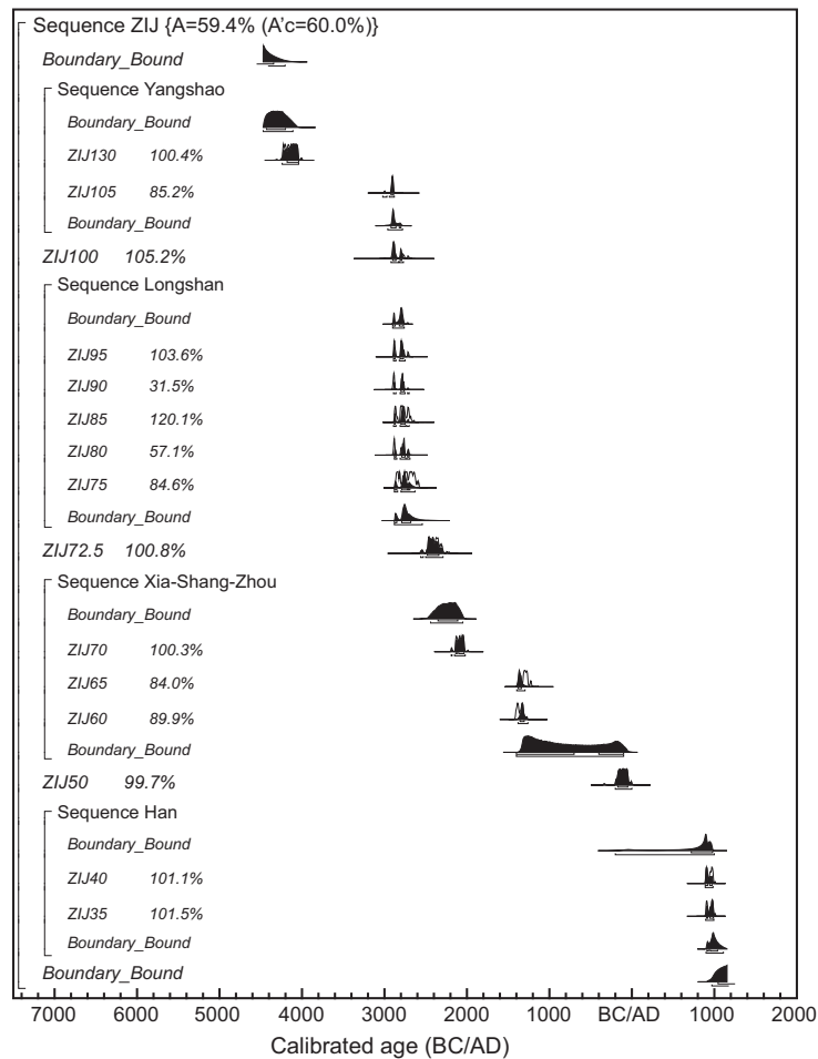
Figure 4 Bayesian tree-ring calibration of sequential ^{14}\text{C} dates for the Zijing site
