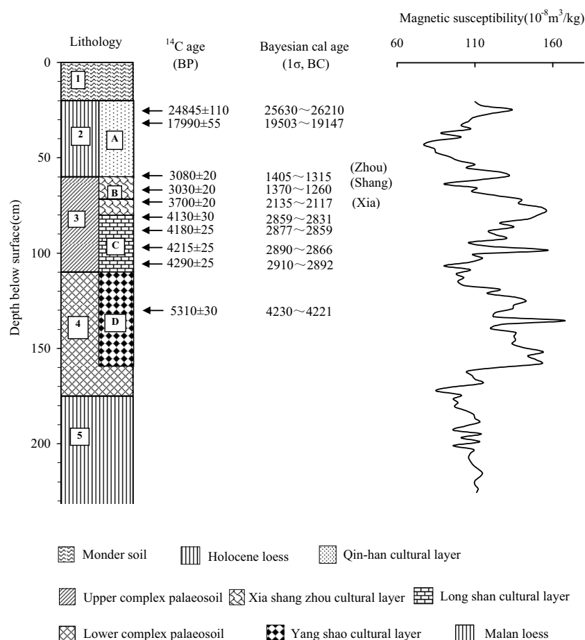
Figure 2 Lithologic and magnetic-susceptibility stratigraphies of the Zijing site. Numbers and letters denote stratigraphical and cultural units, respectively. For details of these units and ^{14}\text{C} dates, see text and Table 2.
