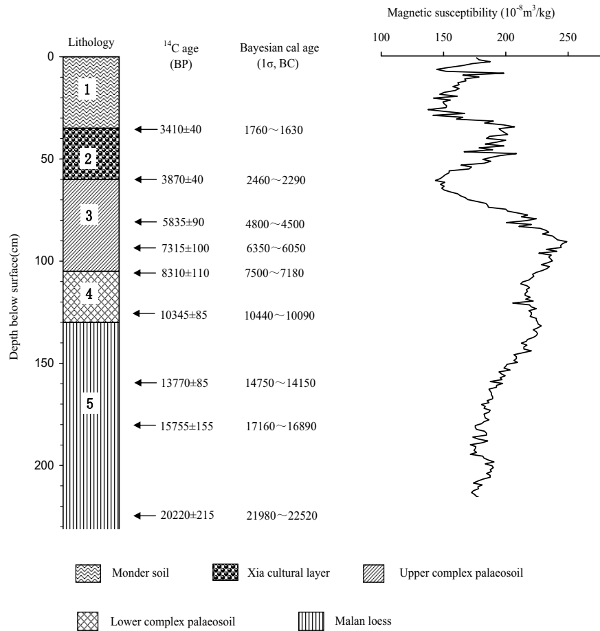
Figure 1 Lithologic and magnetic-susceptibility stratigraphies of the Donglongshan site. Numbers denote stratigraphical units. For details of these units and ^{14}\text{C} dates, see text and Table 1.
