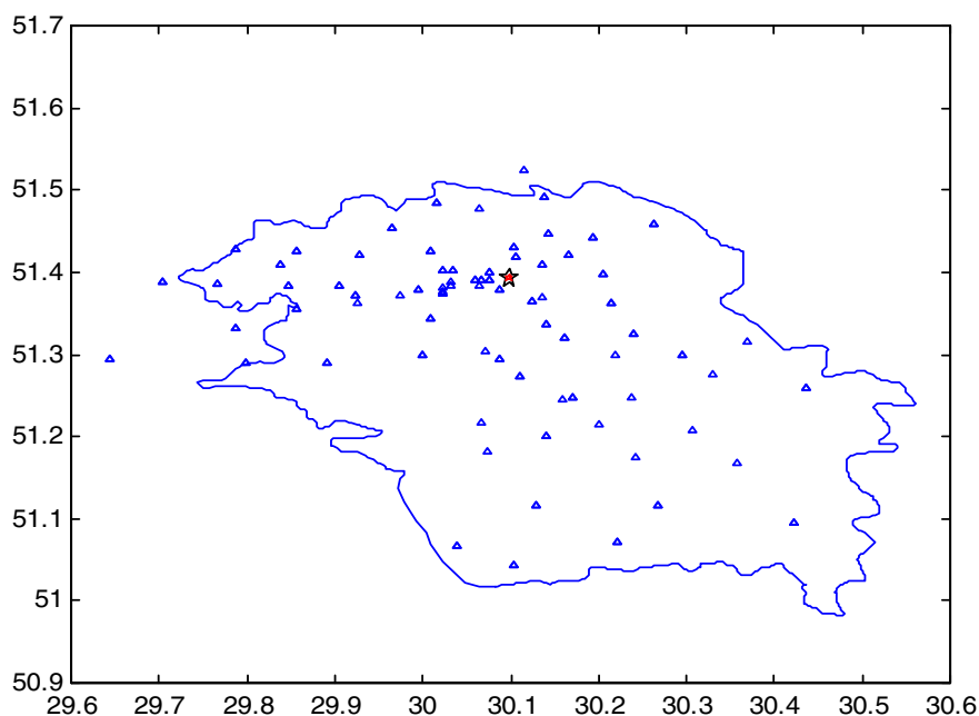
Figure 1 Sampling map for ^{14}\text{C} study (Buzinny et al. 1998; Buzinny and Talerko 1999, 2000a). The border in the map corresponds to border of the former Chernobyl district. The axes represent the latitude and longitude coordinates given in Table 2.
