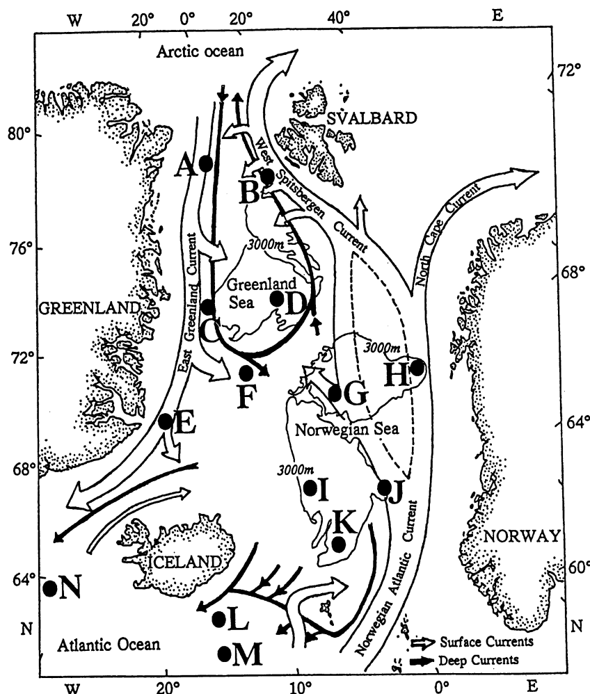
Fig. 4. Map of ^{14}\text{C} depth profiles in the Nordic Seas 1989–1992. The various letters A, B,...N indicate the approximate locations of the ^{14}\text{C} profiles seen in Fig. 5a,b,c,d.
