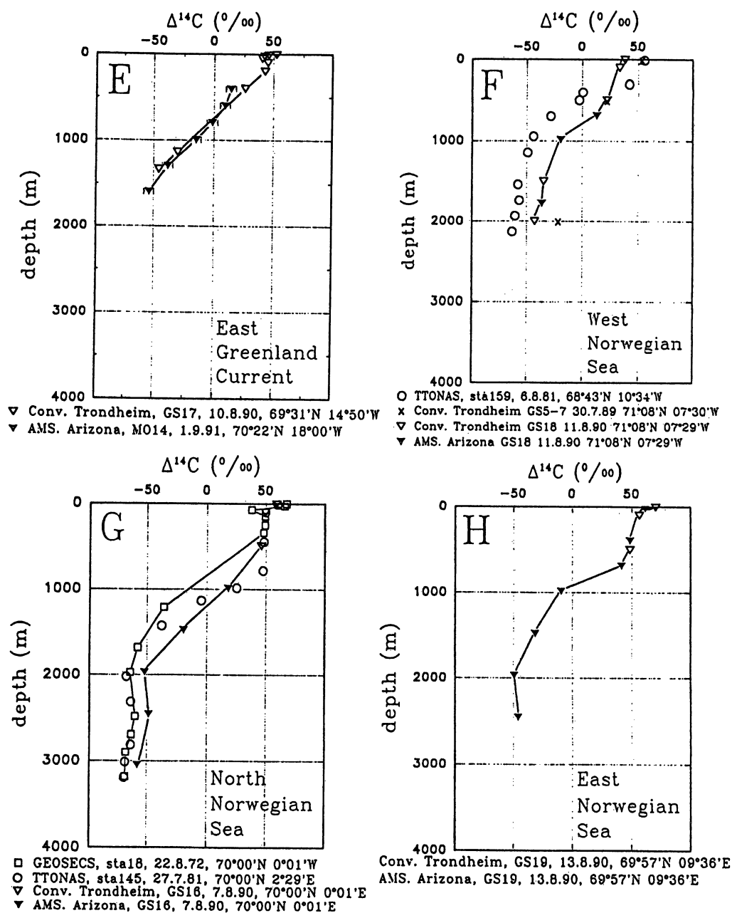
Fig. 5b. ^{14}\text{C} depth profiles in the Norwegian and Icelandic Seas
