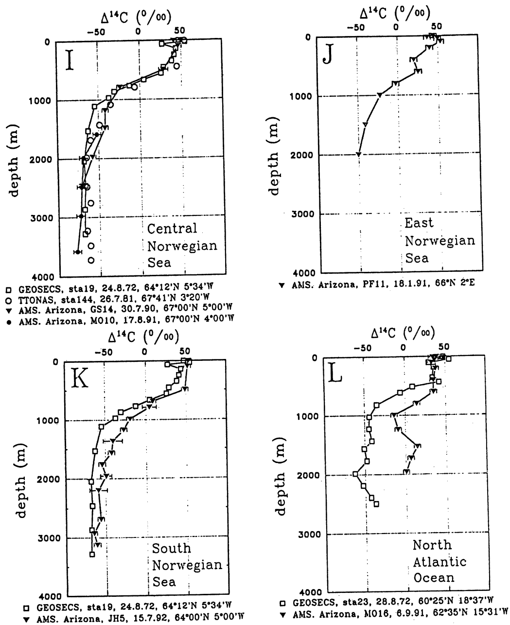
Fig. 5c. ^{14}\text{C} depth profiles from the Norwegian Sea to south of Iceland
