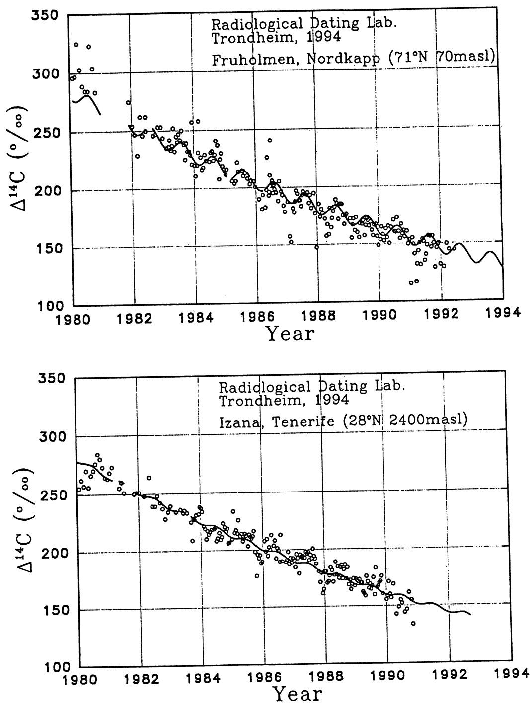
Fig. 2. ^{14}\text{C} in the troposphere at Nordkapp (71°N) and Tenerife (28°N) 1980–1992
