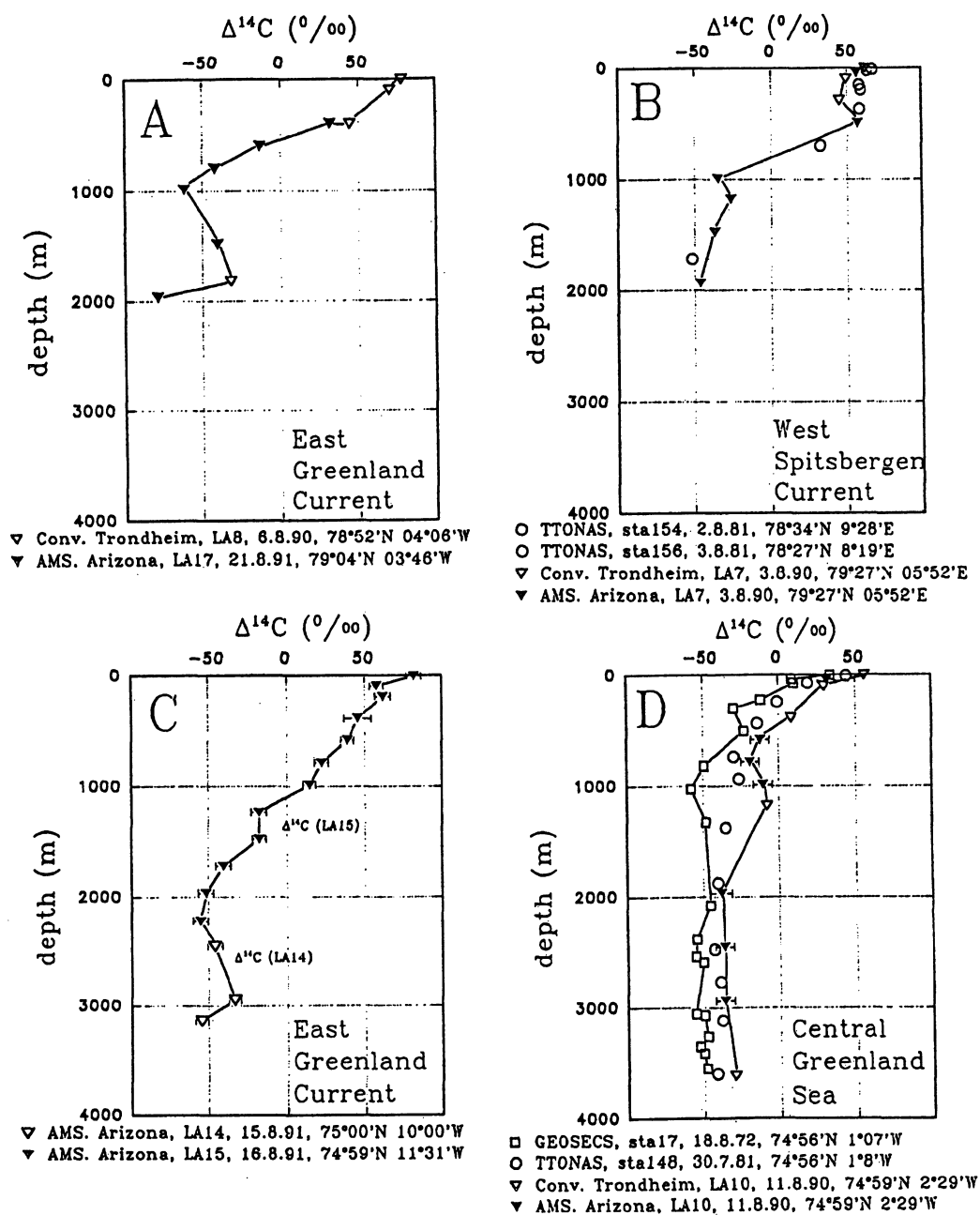
Fig. 5a. ^{14}\text{C} depth profiles in the Greenland Sea
