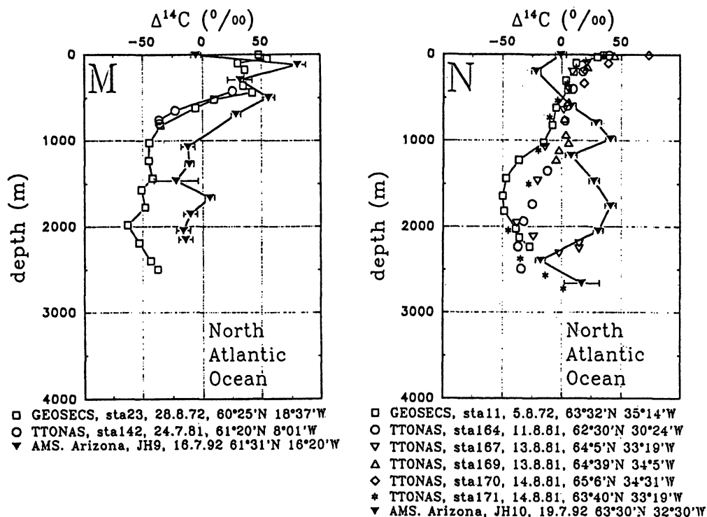
Fig. 5d. ^{14}\text{C} depth profiles in the Atlantic Ocean south of Iceland
