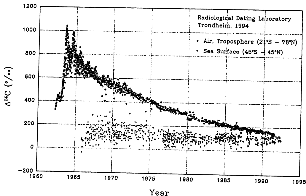
Fig. 1. ^{14}\text{C} in the troposphere and the ocean surface 1962–1992. Measurements only from Nordkapp ( 71^\circ\text{N} ) and Tenerife ( 28^\circ\text{N} ) after 1978.
