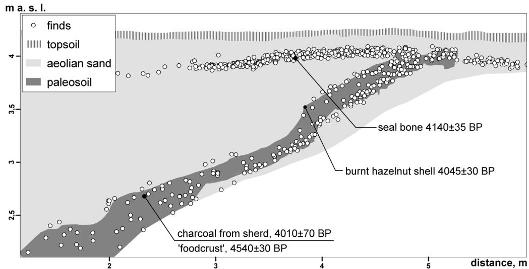
Figure 6 Stratigraphic profile with ^{14}\text{C} -dated Neolithic Rzucewo culture horizons at Nida (2012 research by G Piličiauskas)
