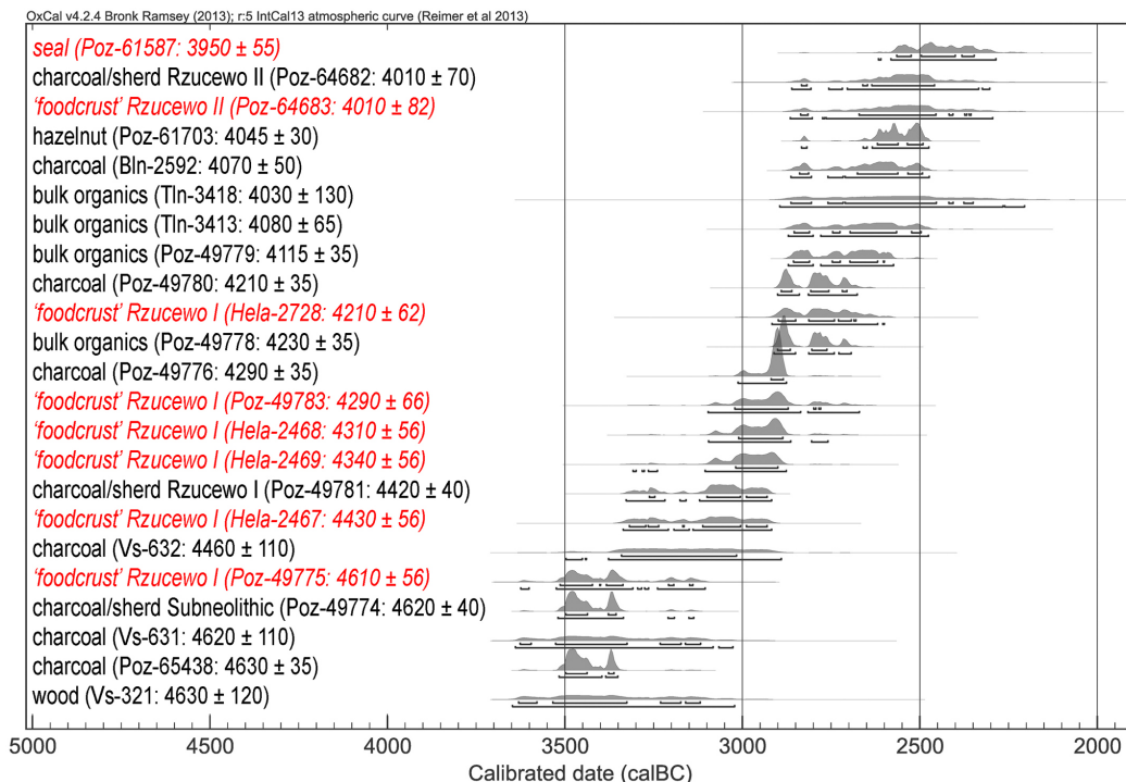
Figure 10 Calibration plot for Nida. ^{14}\text{C} ages corrected for MRE and FROs are marked with red color and italic font. The earliest and latest dates (Le-1361: 11090 \pm 100 ; Vs-320: 3470 \pm 70 ; Le-1384: 3190 \pm 60 ; Le-1976: 2850 \pm 40 ), are inconsistent with archaeological and geological data, and are not included.
