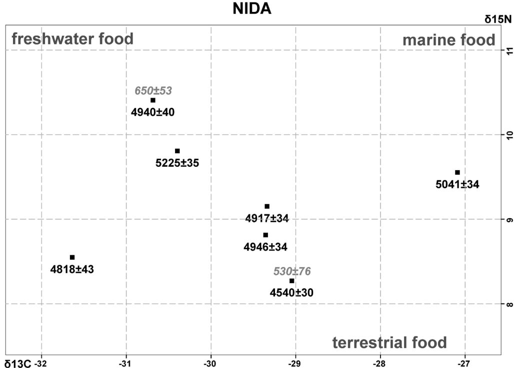
Figure 9 ^{14}\text{C} dates and offsets in the context of bulk stable isotope values of foodcrusts at Nida
