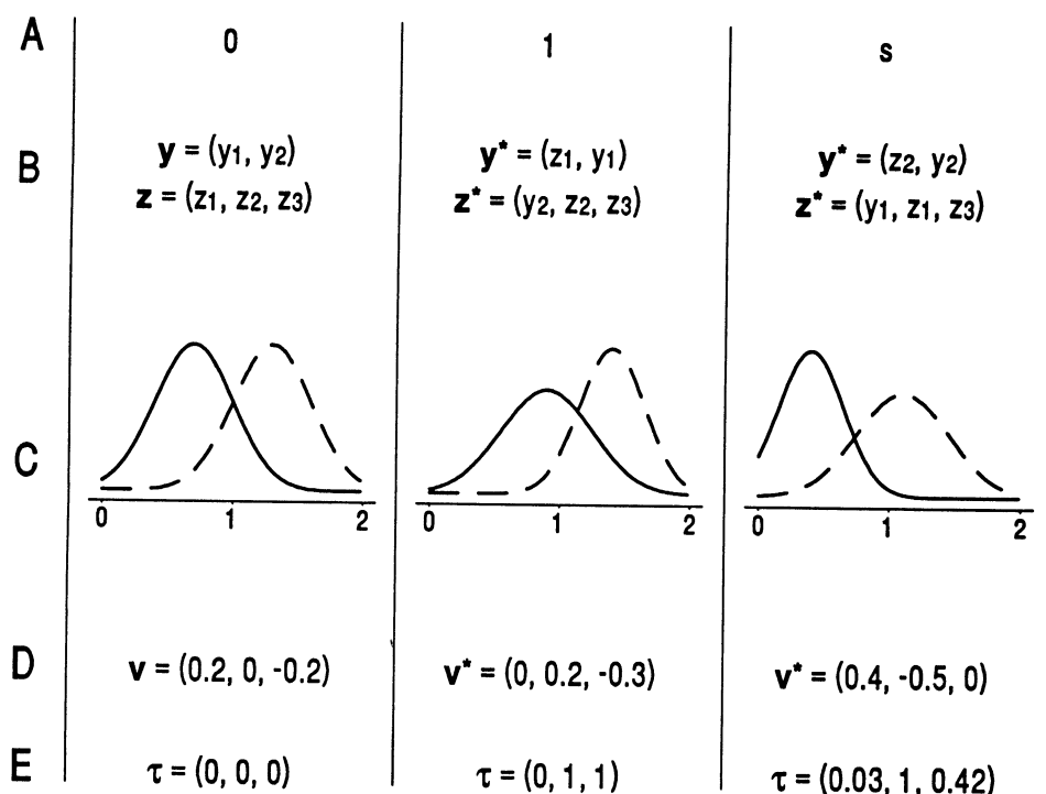
Fig. 1. Schematic illustration of the approximate randomization technique for comparing two ^{14}\text{C} histograms. The left panel shows the original data, the middle panel shows the first shuffle, and the right panel shows the last shuffle. A. Shuffle counter. B. Original (y, z) and simulated (y^*, z^*) ^{14}\text{C} date suites. The individual ^{14}\text{C} dates are shown in abbreviated form; y_1 = y_1 \pm \sigma_1 , etc. C. Calibrated histograms; H_y = solid line, H_z = dashed line. The x-axis shows years 0, 1, and 2. D. The actual ( v ) and simulated ( v^* ) test statistics for years 0, 1, and 2. E. Estimated significance of the actual test statistic. The 0 values in the left panel indicate no estimate of significance. In the right panel the actual statistic at year 0 is significant at \alpha < 0.05 .
