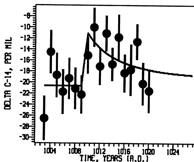
Fig. 3. Measurements of \Delta^{14}\text{C} (age and stable isotope-corrected deviations from a standard value). Precision is \pm 1\sigma . The curve is a six-box carbon model with sedimentary sink fit to the data, assuming the \gamma -rays ( >10 MeV) arrive as a pulse immediately after AD 1009. A pulse lasting 2 yr provides an equally good fit to the data.
