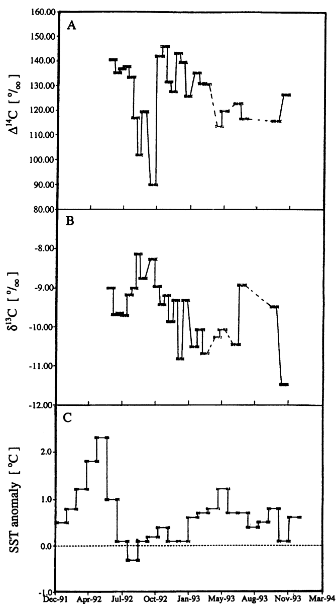
Fig. 3. Record of (A) \Delta^{14}\text{C} and (B) \delta^{13}\text{C} of atmospheric \text{CO}_2 collected at the Aychapicho, Ecuador station ( 0.11^\circ\text{S} , 78.85^\circ\text{W} , 2996 m asl). Data points represent two-week composite samples. (C) Record of monthly mean SST anomaly off the coast of Peru and Ecuador during 1992 and 1993 (WMO 1994). The record can be considered a proxy indicator of the intensity of upwelling: high positive anomaly indicates occurrence of the ENSO event and suppressed upwelling in the eastern Pacific.
