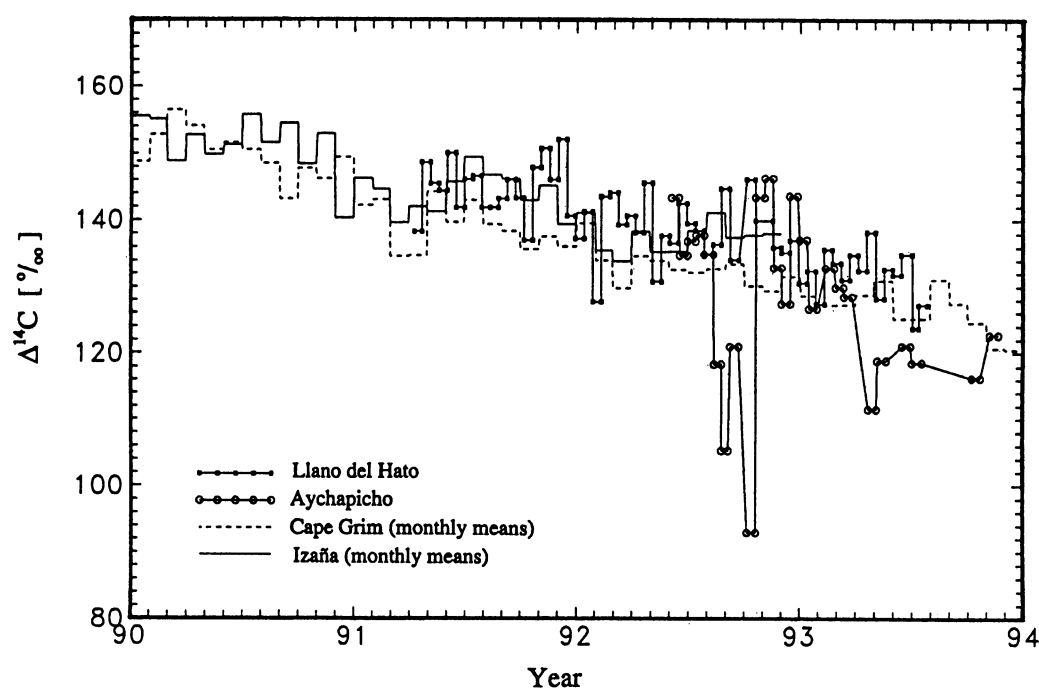
Fig. 2. Atmospheric ^{14}\text{CO}_2 levels monitored at four stations shown in Figure 1, which represent the tropical region and mid-latitudes of both hemispheres: Llano del Hato, Venezuela ( 8^\circ\text{N} , 72^\circ\text{W} , 3600 m asl), Aychapicho, Ecuador ( 0.11^\circ\text{S} , 78.85^\circ\text{W} , 2996 m asl), Izaña, Tenerife, Spain ( 28^\circ\text{N} , 16^\circ\text{W} , 2376 m asl) and Cape Grim, Tasmania ( 41^\circ\text{S} , 145^\circ\text{E} , 95 m asl)
