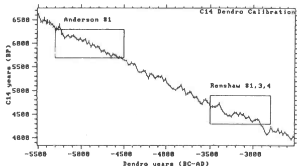
Fig. 3. Part of the dendrochronological calibration curve with the regions of interest emphasized
