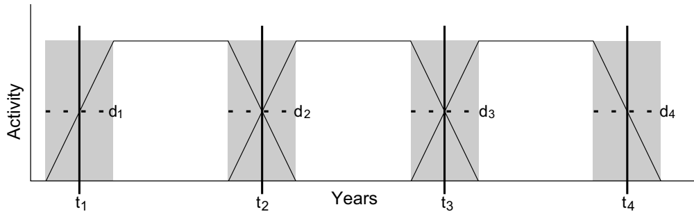
Figure 4 Schematic diagram showing the use of the trapezoid in a very specific contiguous multiphase trapezoid model. The thick vertical lines are the boundaries and the dotted horizontal lines are transitions. The transition parameters can be used to estimate the duration of transition between any 2 phases, highlighted in gray.
