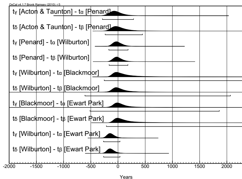
Figure 12 Estimates for the overlap between the rise and decline of adjacent phases at 95.4% confidence; negative values here indicate a gap in years between the specified parameters and positive values indicate an overlap.
