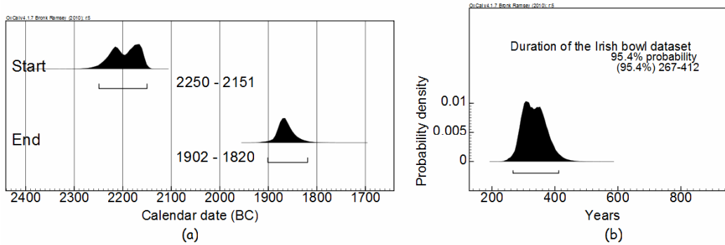
Figure 2 Probability density functions of the (a) uniform parameters and (b) timespan of the model at 95.4% confidence
