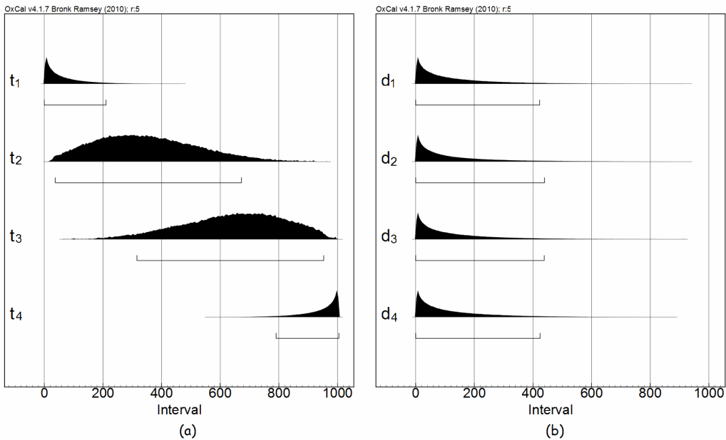
Figure 8 Marginal distributions of the (a) trapezoid boundaries and (b) transitions under Equation 4 for 3 contiguous phases with 10 events. The timespan ( S ) of the model is constrained to be 1000.
