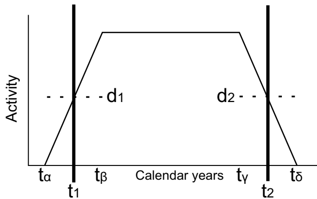
Figure 3 Schematic representation of the trapezoid prior model (Karlsberg 2006), where activity relates to usage, deposition, or production rate. The thick vertical lines are boundaries, t_1 and t_2 , and the dotted horizontal lines are transitions, d_1 and d_2 . t_\alpha , t_\beta , t_\gamma , and t_\delta are Karlsberg’s parameters for the model, where \alpha = t_1 - d_1/2 , \beta = t_1 + d_1/2 , \gamma = t_2 - d_2/2 , and \delta = t_2 + d_2/2 .
