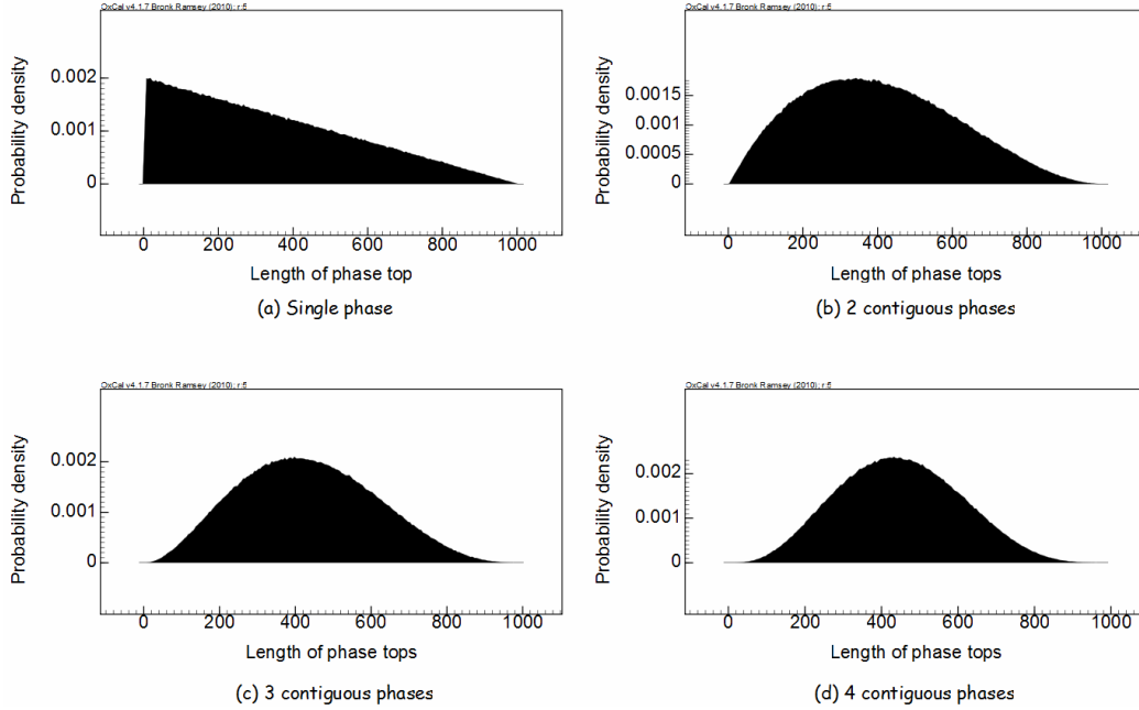
Figure 5 Probability distributions of the sum of phase tops ( \mathbb{T} ) under Equation 2 for up to 4 contiguous phases. The timespan ( S ) of the model is constrained to be 1000.
