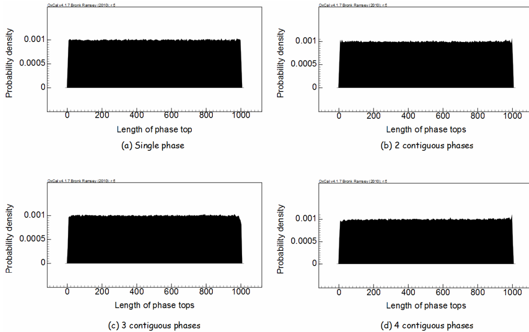
Figure 6 Probability distributions of the sum of phase tops ( T ) under Equation 4 for up to 4 contiguous phases. The timespan ( S ) of the model is constrained to be 1000.
