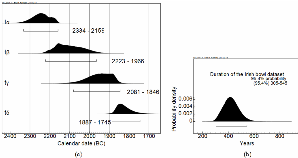
Figure 9 Probability density functions of the (a) trapezoid parameters and (b) timespan of the model, under Equation 4, at 95.4% confidence.
