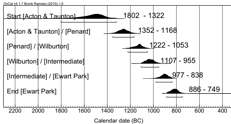
Figure 15 Probability density functions of the estimated calendar dates of transition between the Bronze Age phases at 95.4% confidence, modeled using contiguous uniform phases.
