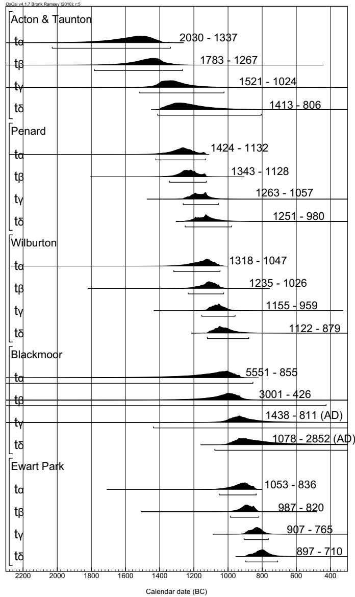
Figure 11 Probability density function of the trapezoid parameters for the Bronze Age phases, under Equation 4, at 95.4% confidence.
