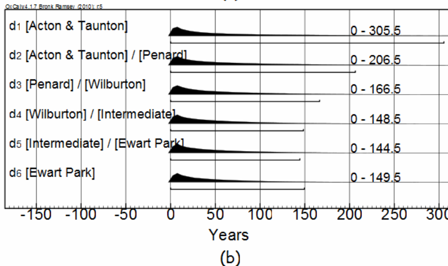
Figure 14 Probability density functions of the (a) trapezoid boundaries and (b) transitions for the Bronze Age phases, under Equation 4, at 95.4% confidence.
