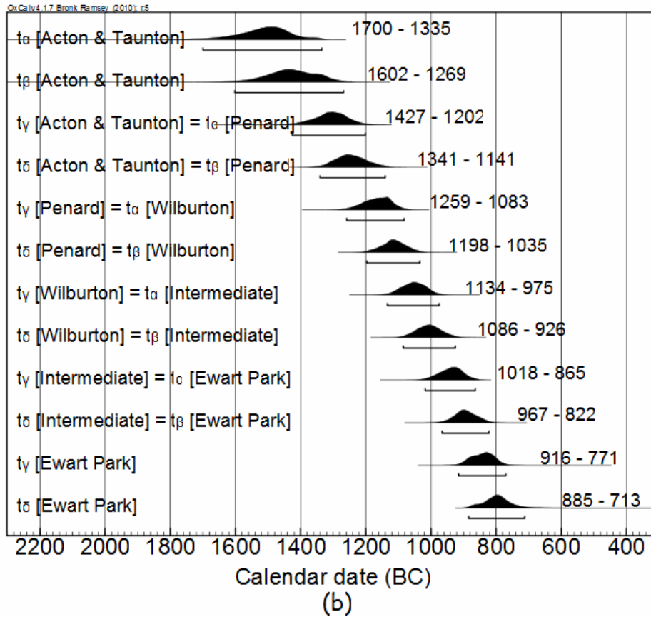
Figure 13 Model B: (a) the prior assumptions with the abbreviated phases in the square brackets; and (b) probability density functions of the trapezoid parameters for the Bronze Age phases, under Equation 4, at 95.4% confidence.
