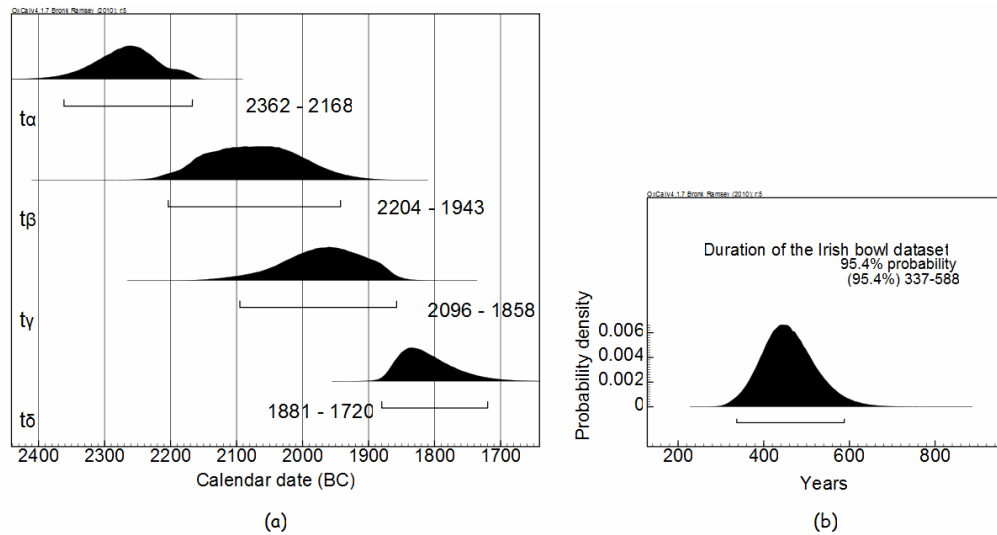
Figure 1 Probability density functions of the (a) trapezoid parameters and (b) timespan of the model at 95.4% confidence
