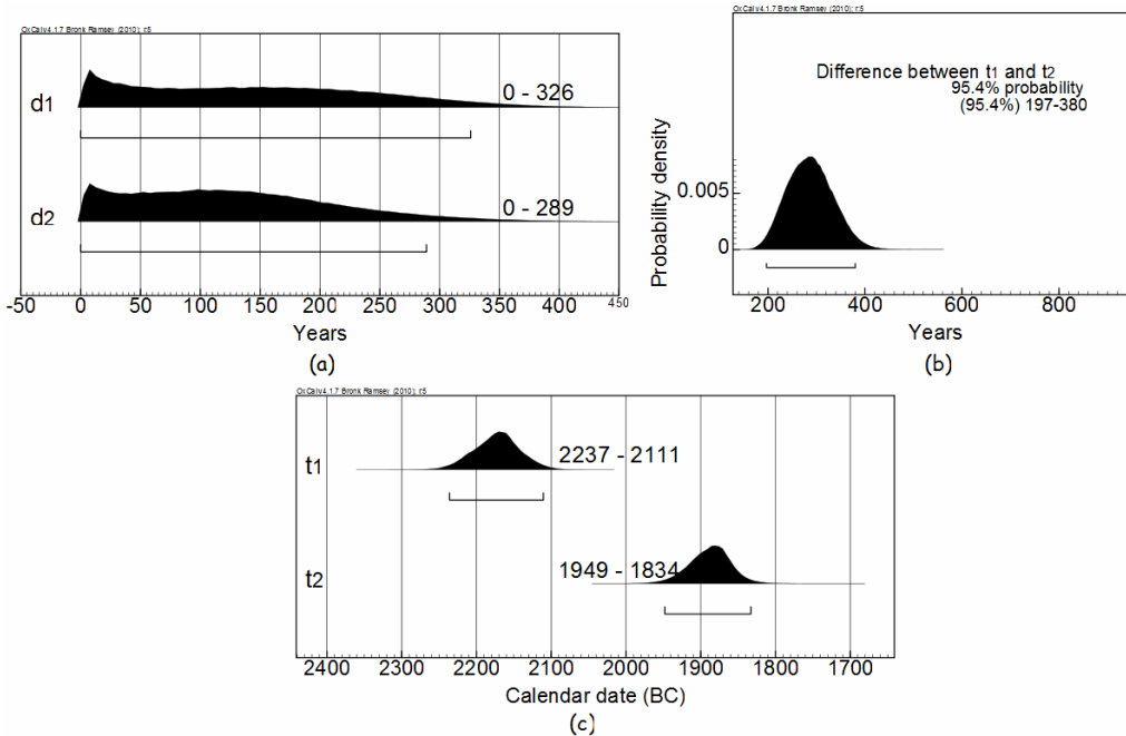
Figure 10 Probability density functions of the (a) new trapezoid parameters; (b) the difference between the boundary parameters t_1 and t_2 ; and (c) timespan of the model, under Equation 4 at 95.4% confidence.
