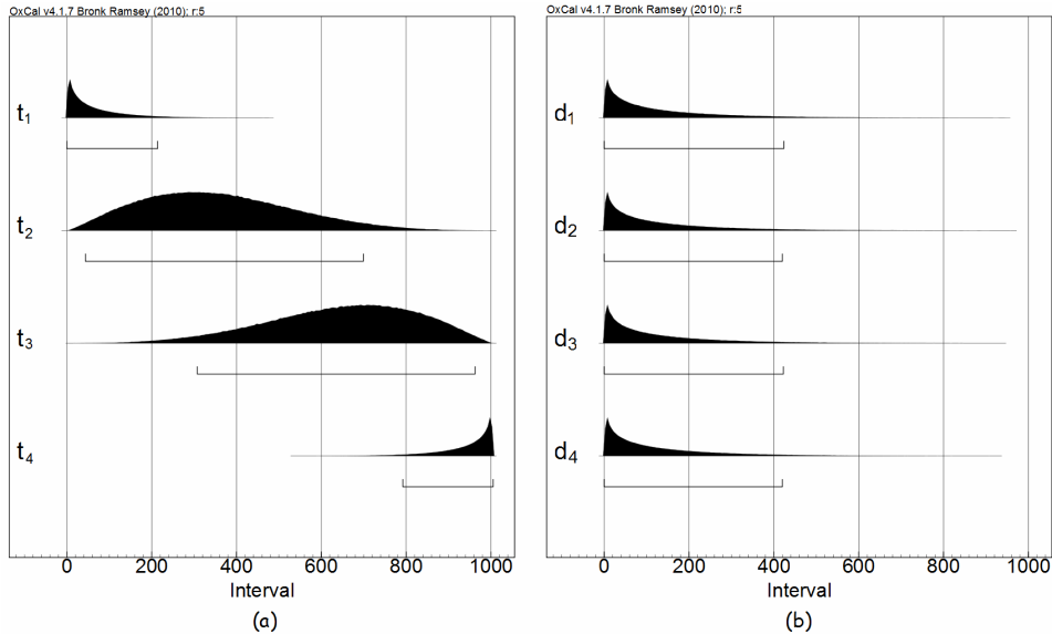
Figure 7 Marginal distributions of the (a) trapezoid boundaries and (b) transitions under Equation 4 for 3 contiguous phases with no events. The timespan ( S ) of the model is constrained to be 1000.
