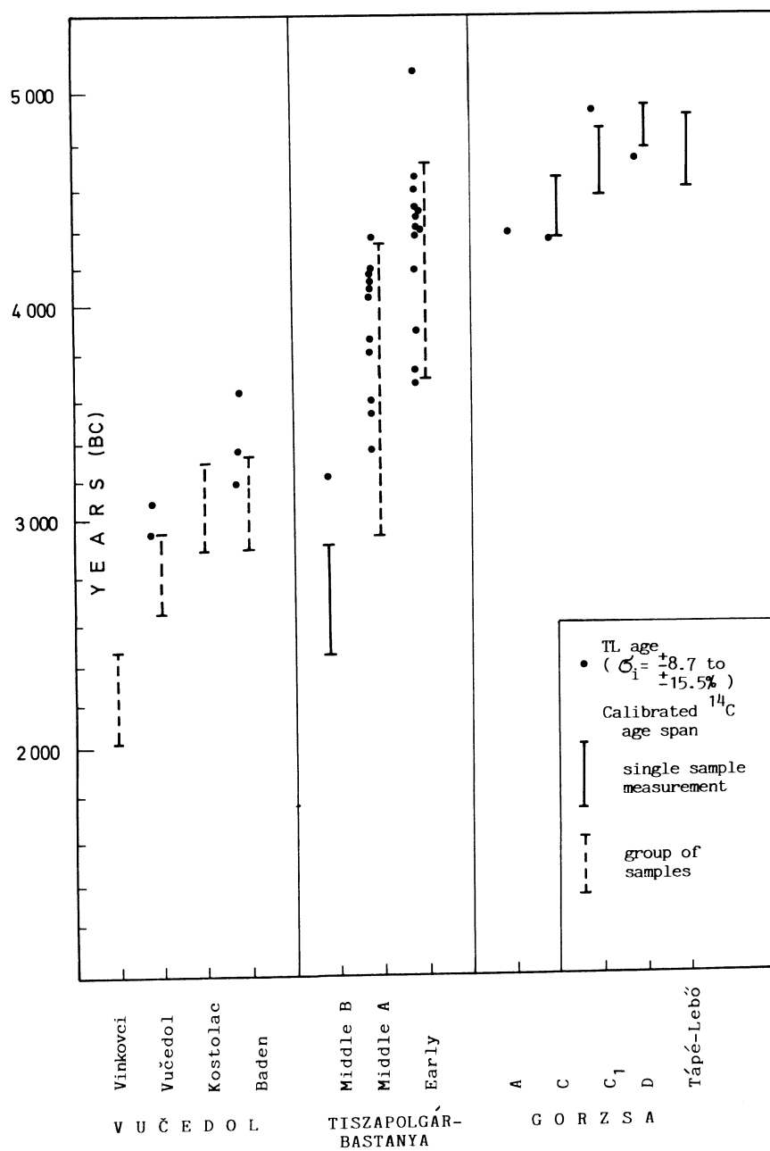
Fig 6. Comparison of TL and calibrated ^{14}\text{C} dates
