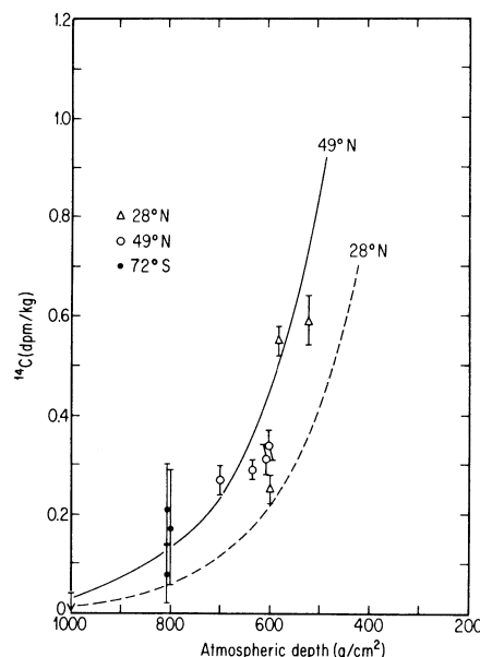
Fig 1. ^{14}\text{C} (dpm/kg) measured in rocks of different altitude (plotted as atmospheric depth in \text{g}/\text{cm}^2 ) and geomagnetic latitude
