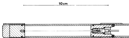
Fig 2. The prototype proportional gas counter. In this version the gas is admitted to and evacuated through the spring cavity, the gas capillary serving as the HV lead at the same time.
