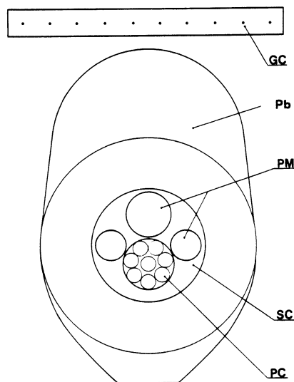
Fig 1. A cross-sectional view of the multicounter shield consisting of: gas-proportional flow counter (GC), massive asymmetric lead shield (Pb), photomultipliers (PM) facing plastic scintillator (SC) and sample gas-proportional counters (PC). The copper and cadmium layers as described in the text are not shown.
