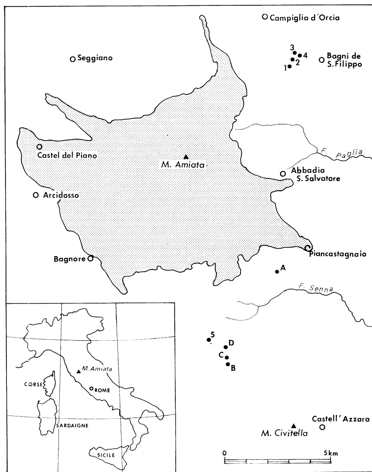
Fig 1. Position of analyzed samples (letters: mofettes; figures: plants; shaded area: Mte Amiata volcanics).
