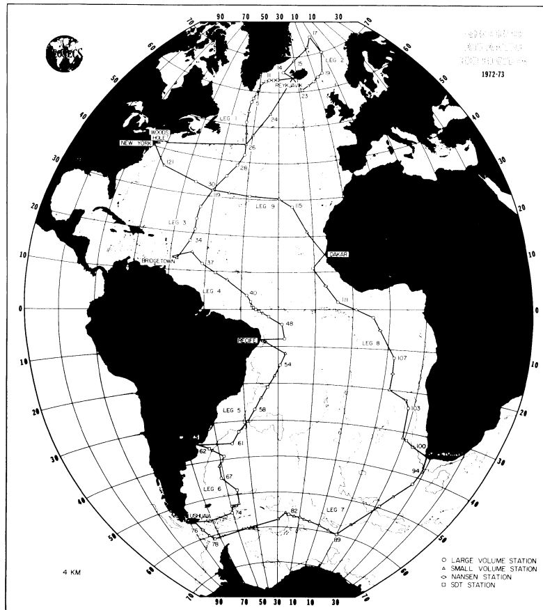
Fig 1. GEOSECS Atlantic Track 1972-1973.
