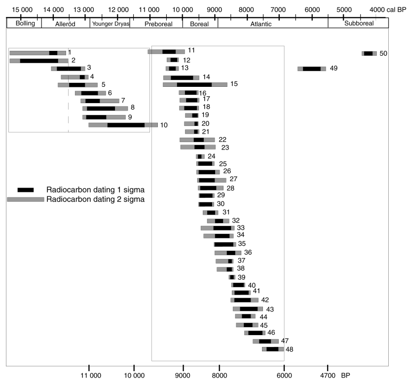
Figure 2 ^{14}\text{C} dates of Holocene subfossil trunks from the middle Durance basin. All the dates are calibrated with INTCAL98 (Stuiver et al. 1998). Most of the trees are buried in alluvial deposits during a time span from Allerød to Atlantic. For location and reference see Table 1 and Figure 1.
