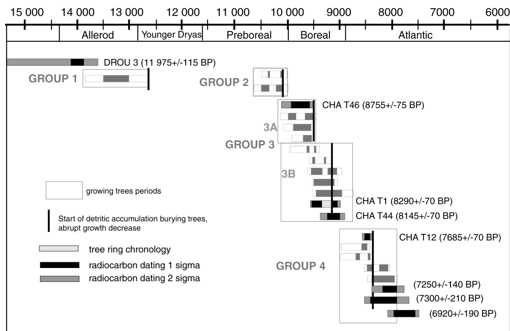
Figure 5 ^{14}\text{C} dates of Drouzet subfossil trunks and Saignon subfossil trunks (in gray). All the dates are calibrated with INTCAL98 (Stuiver et al. 1998). The dates in the Drouzet basin are from the same time interval as those from the Saignon. This suggests that tree growing periods are simultaneous in the two basins.
