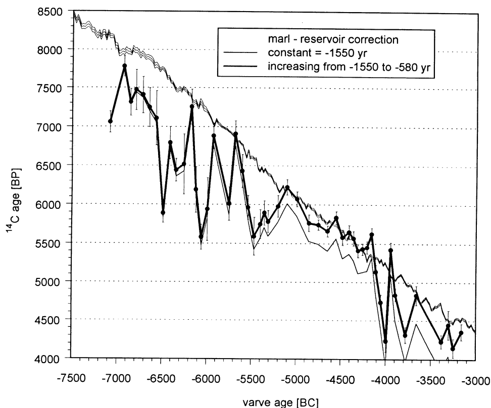
Fig. 6. Calibration curve and reservoir-corrected ^{14}\text{C} ages of the marl fraction from sediments in Schleinssee (Geyh, Merkt and Müller 1971). The best fit is obtained with an initial ^{14}\text{C} value that undergoes secular change (bold line) starting with -1550 yr for 9000 BP and ending with -580 yr at present. A constant initial ^{14}\text{C} value yields a worse fit.
