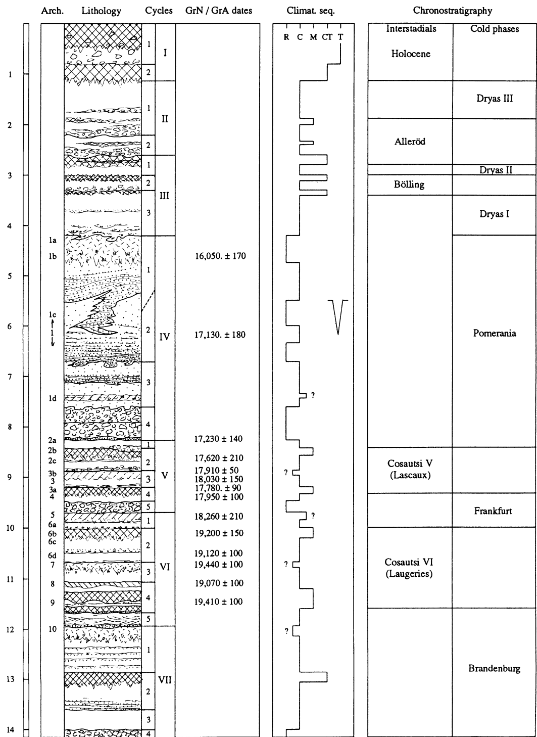
Fig. 2. Stratigraphy, chronology, climatic sequence and chronostratigraphy of the Cosautsi site. Climatic sequence: R = rigorous, C = cold, M = medium cold, CT = cold-temperate, T = temperate.
