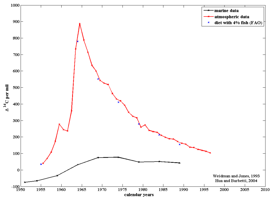
Figure 2 Atmospheric, marine and dietary curve of ^{14}\text{C} data for Georges Bank
