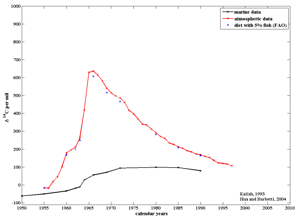
Figure 3 Atmospheric, marine and dietary curve of ^{14}\text{C} data for New Zealand
