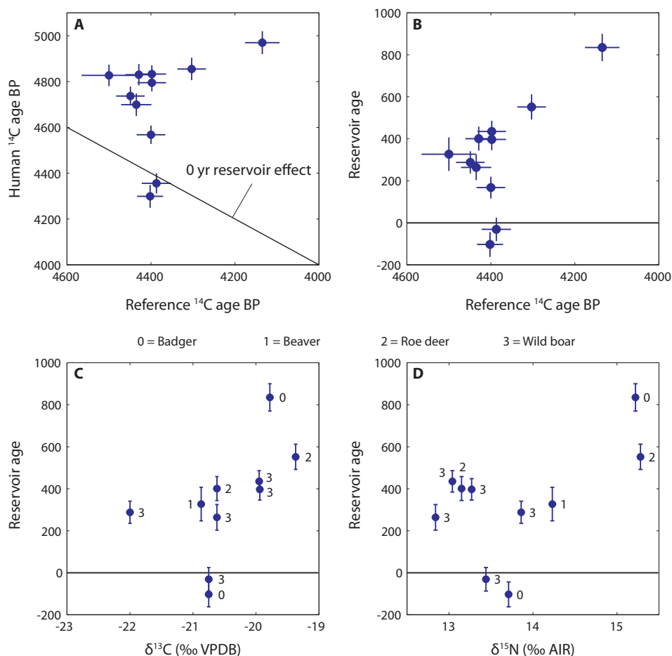
Figure 5 A) Measured human ^{14}\text{C} ages versus the associated terrestrial animal tooth pendant ^{14}\text{C} age (reference age). The solid black line indicates no reservoir effect, i.e. similar animal tooth pendant and human ^{14}\text{C} age ( x = y line). Note that the reservoir age is calculated as the vertical distance from the no reservoir effect line to the human ^{14}\text{C} age. B) Associated terrestrial animal tooth pendant ^{14}\text{C} age (reference age) versus calculated reservoir age R. C) The human \delta^{13}\text{C} values versus the calculated reservoir age. D) The human \delta^{15}\text{N} values versus the calculated reservoir age R. For each data point in C and D the species of the reference animal is indicated by a number.
