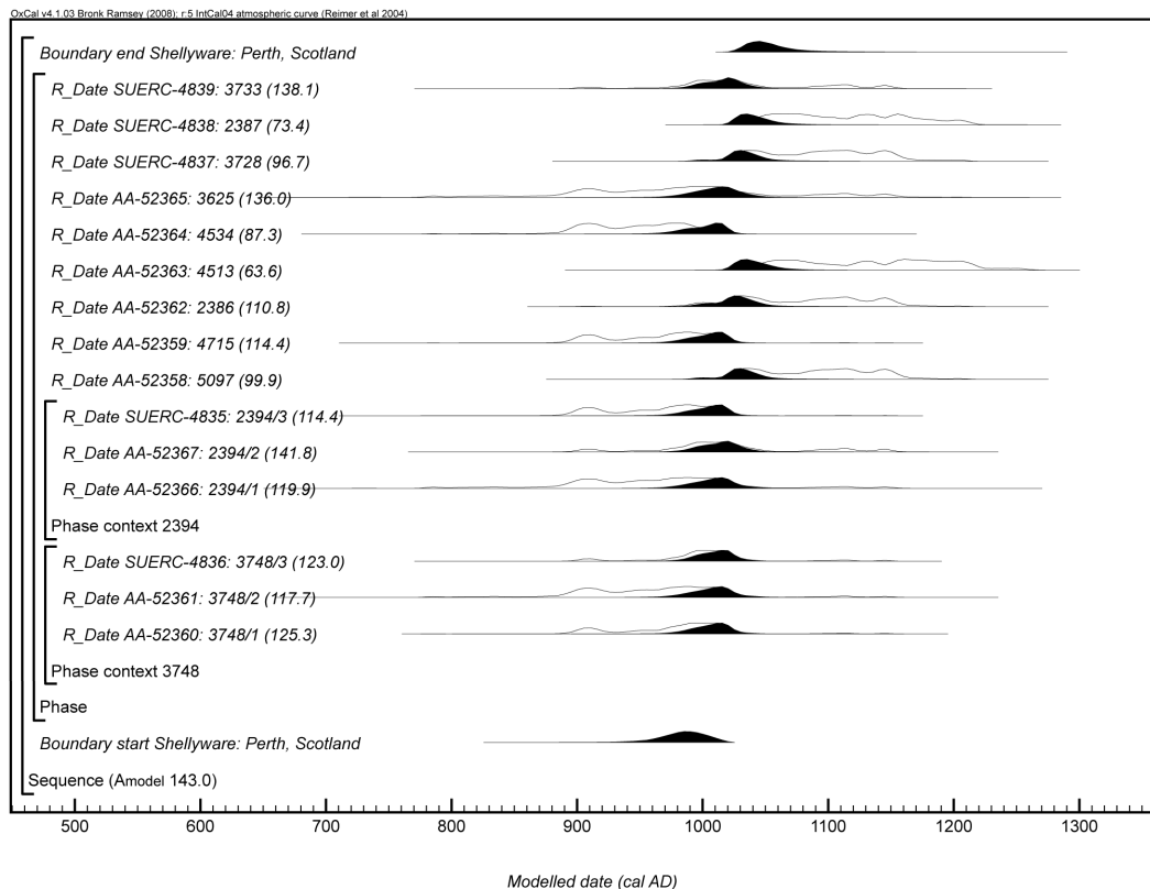
Figure 1 Graphical representation of the calibration of ^{14}\text{C} results for carbonized residues on London Sandy Shellyware from Perth, Scotland.
