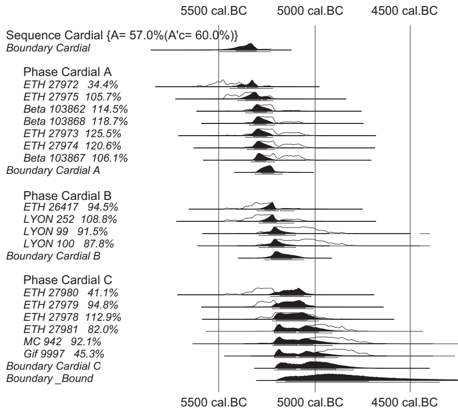
Figure 5 Results of Bayesian Phase model applied to Groups A, B, and C
