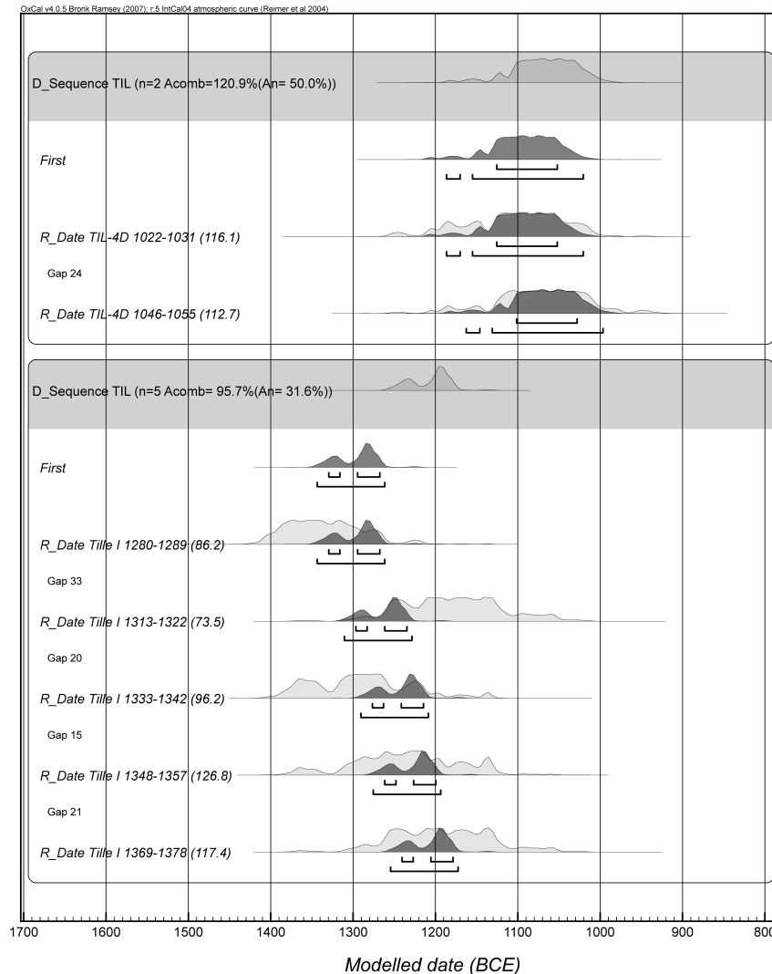
Figure 5 Modeled calendar age BCE placements of the ^{14}\text{C} -dated samples from Tille Höyük given the known dendrochronological spacings between the samples from each of the 3 dated sequences. Data from OxCal (Bronk Ramsey 1995, 2001, 2008 v 4.05 with curve resolution set at 5) and IntCal04 (Reimer et al. 2004). The hollow distributions for each individual date show the calibrated probabilities in isolation (no model), and the solid distributions show the reduced probability distributions after applying the Defined Sequence analysis model. The upper and lower lines under each distribution show the respective 1- \sigma (68.2% confidence) and 2- \sigma (95.4% confidence) calibrated age ranges (for the modeled results): see Table 2 (which gives the 1- and 2- \sigma ranges).
