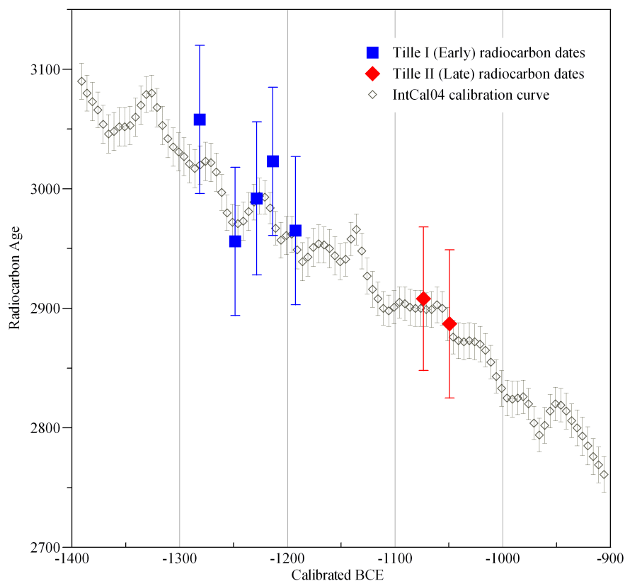
Figure 4 Placement of the 7 Tille Höyük ^{14}\text{C} measurements against the IntCal04 ^{14}\text{C} calibration curve and in terms of the new Tille Höyük 2008 (Tille08) I (Early) and II (Late) tree-ring chronologies. The wiggle-match fit points shown for the Tille I dates are the centers of the more likely subranges of the 1- \sigma ranges (the most likely 52.3% of the total probability ranges) in Table 2, with the fit error employed being the limits of this subrange. The Tille II (TIL-4D) data are fitted to the middle of their 1- \sigma ranges in Table 2.
