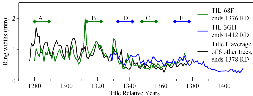
Figure 2 The Tille I chronology constituents, representing TIL-68EFH, TIL-3GH, and the average of all other samples. TIL-68 and TIL-3 are the 2 samples that had ring segments ^{14}\text{C} dated; the segments are indicated as horizontal lines A, B, and C from TIL-68FH, and D and E from TIL-3G. See Tables 1 and 2 and Figures 3–5 for more information about the ^{14}\text{C} ages.
