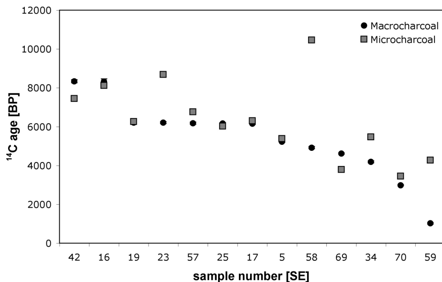
Figure 1 Uncalibrated ^{14}\text{C} ages (BP) of macrocharcoal particles ( >1 mm) and microcharcoal chemically separated from labile soil organic matter by UV photo-oxidation. Both charcoal samples were taken from the same soil sample. The error bars are too small to be shown.
