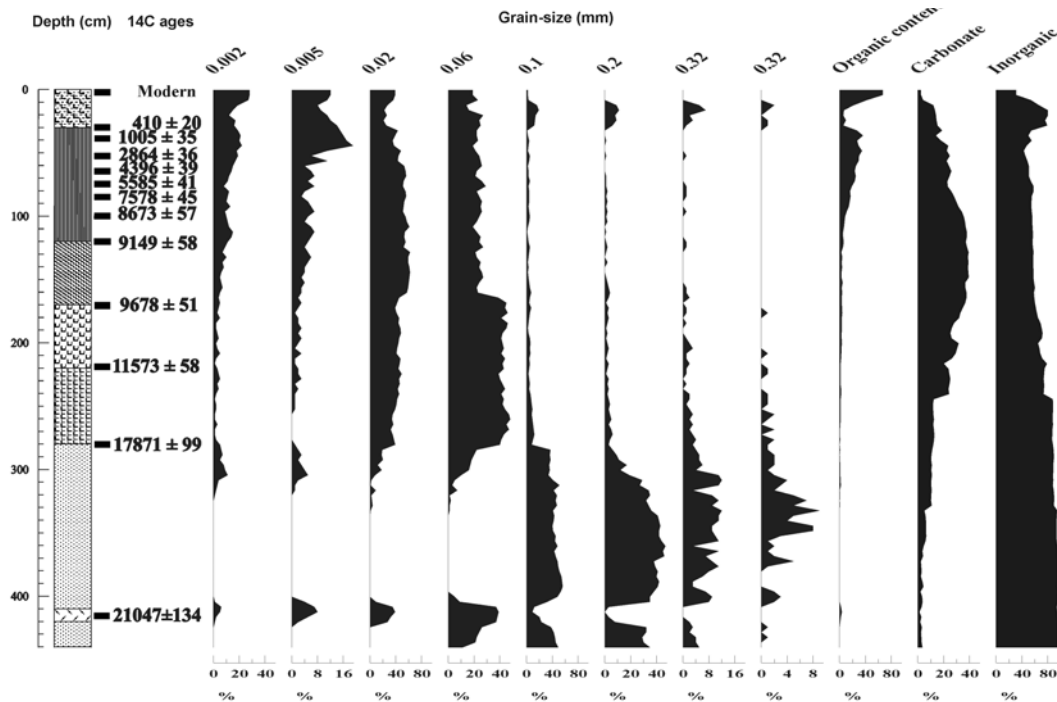
Figure 2 Results of grain-size analysis and loss on ignition (LOI) for the 14 C-dated core 11
