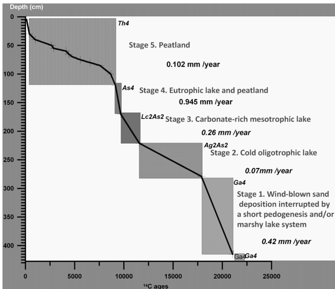
Figure 4 The inferred rate of sedimentation for individual stages of the lake's evolution
