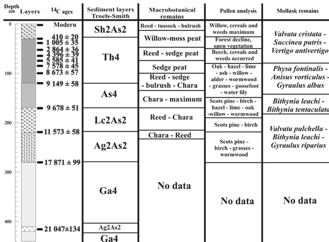
Figure 3 Results of sedimentological, plant macrofossil, palynological, and malacological analyses for the 14 C-dated core 11
