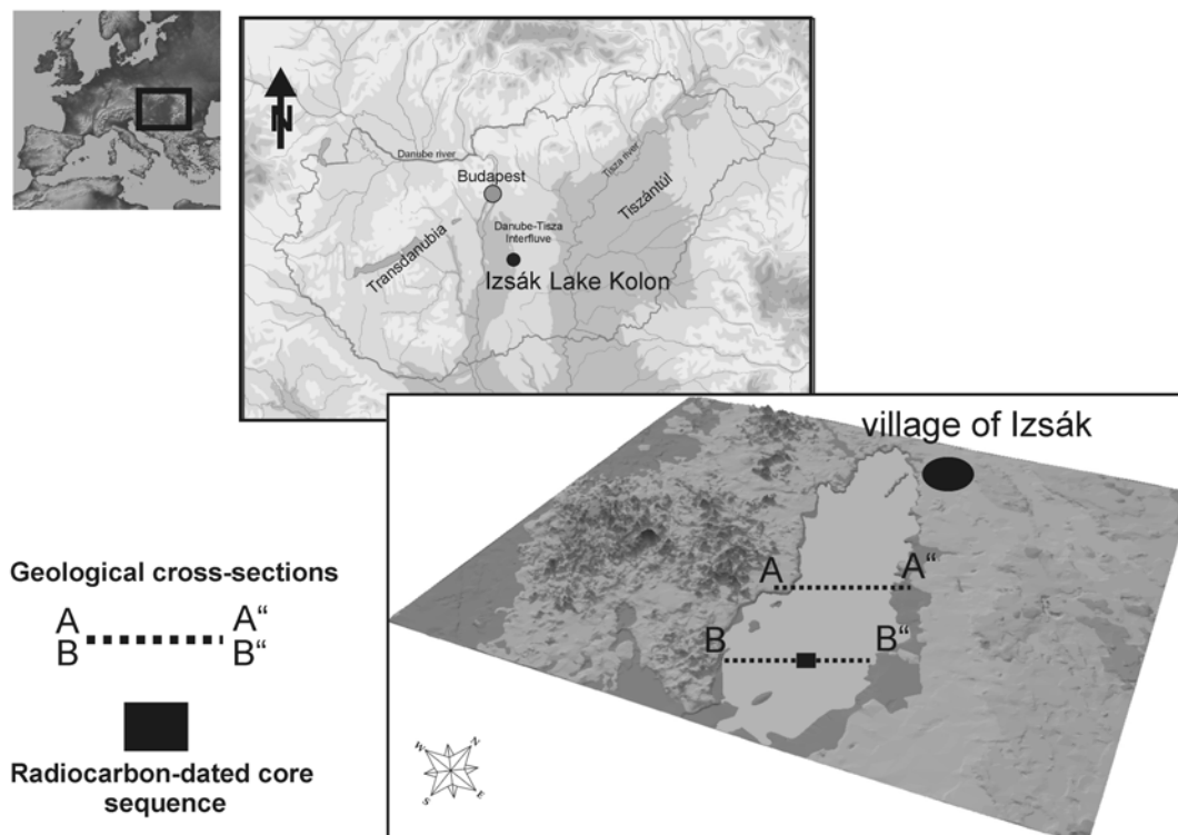
Figure 1 Geographical location of the catchment basin of Lake Kolon in the Danube Valley and the coring site
