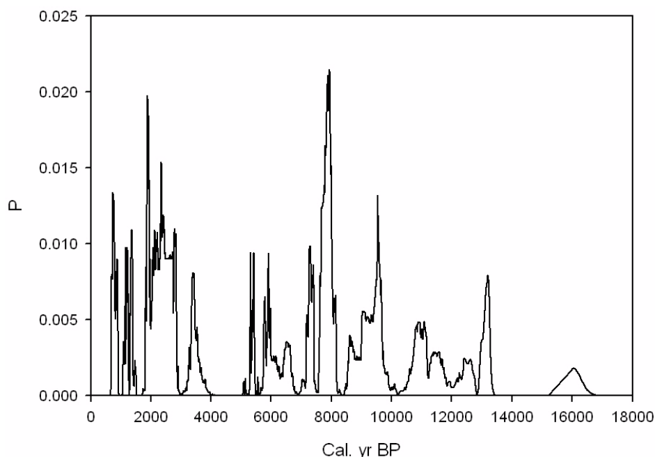
Figure 6 Plot of combined probability distributions (calculated from IntCal 98, Stuiver et al. 1998) for the last 16,000 yr of forest fires at Bear Flat, BC. The probability shown on the vertical axis is from the sum of the ^{14}\text{C} probability curves (Reimer et al. 2004).
