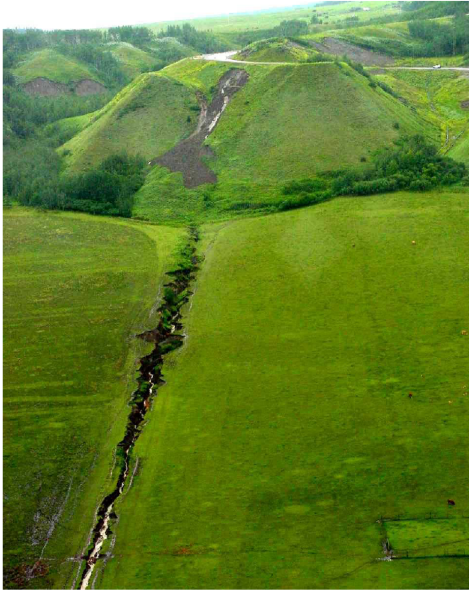
Figure 1 Oblique aerial photograph of the alluvial fan at Bear Flat, BC
