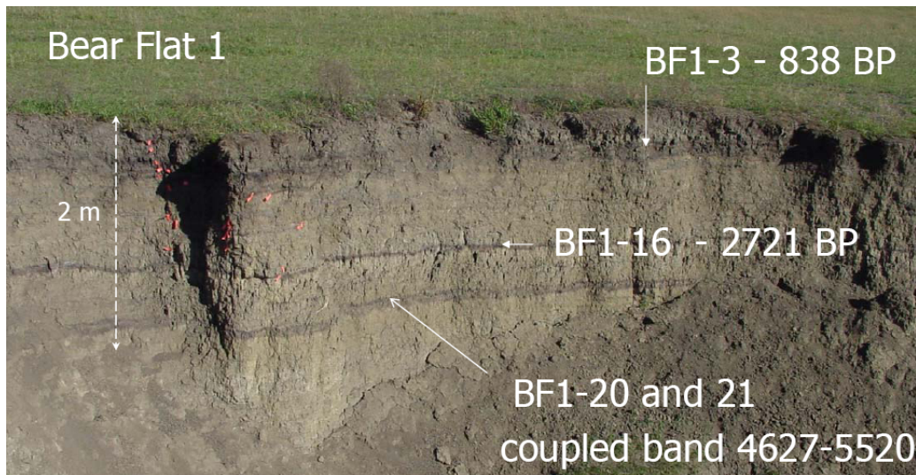
Figure 4 View of the exposure of the buried fire horizons at the Bear Flat 1 location. Discrete charcoal horizons are marked with the red tags, and major fire events are clearly visible in this photograph.
