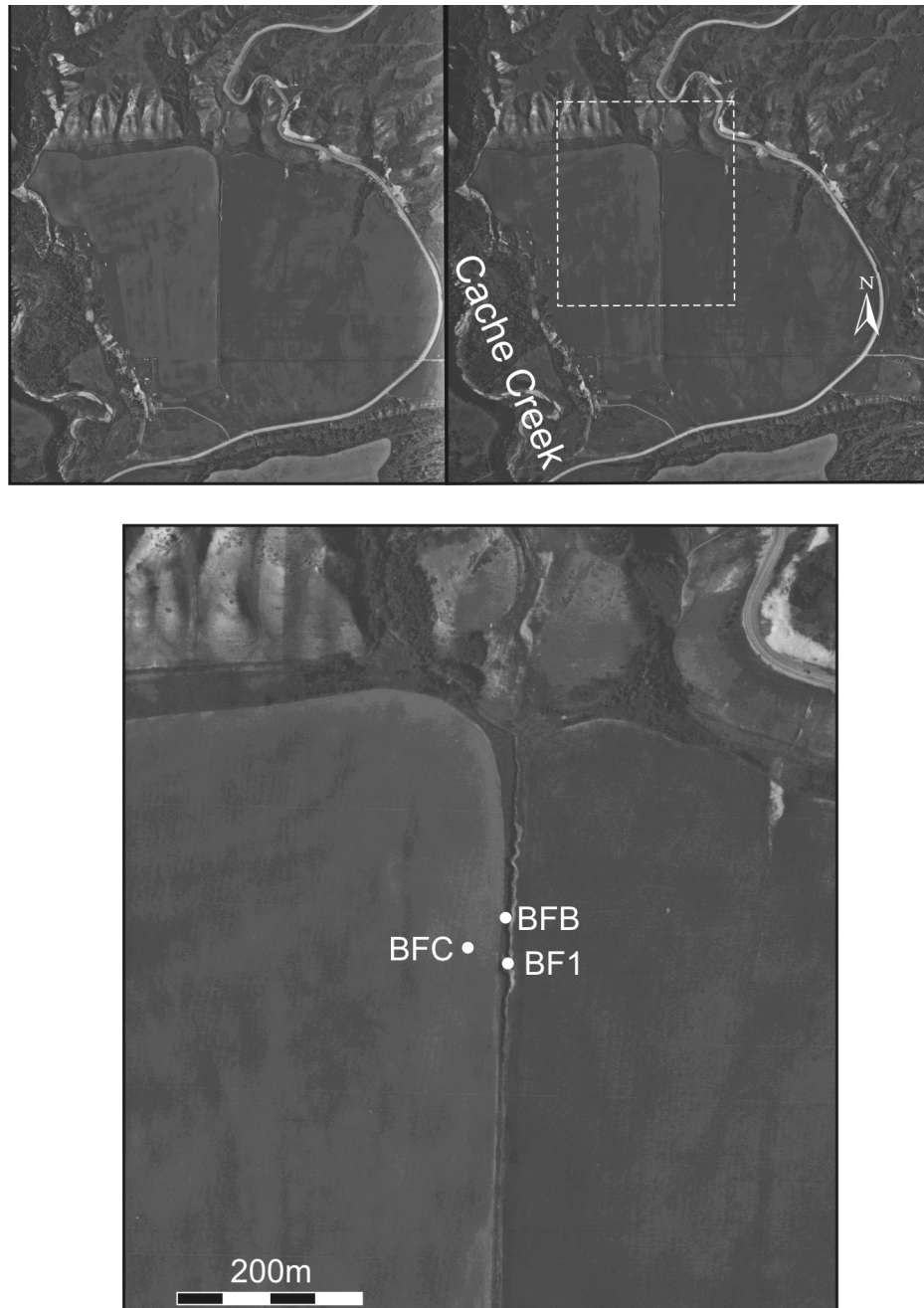
Figure 3 a) Stereo image of the Bear Flat site. b) Detailed view of the Bear Flat fan showing the specific locations of the 3 cores: BF1, BFB, and BFC.
