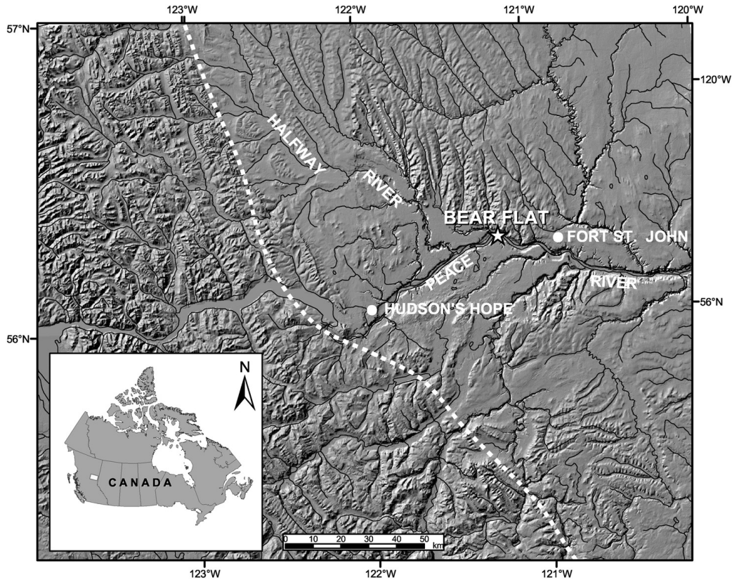
Figure 2 Location of Bear Flat adjacent to the Peace River, northern BC. Note the location of the maximum western extent of the Laurentide ice sheet (dotted line), estimated by Catto et al. (1996) from the distribution of Laurentide erratics. These authors also reported a ^{14}\text{C} date on wood charcoal, from the contact of Laurentide till and overlying Glacial Lake Peace sediments in the Fort St. John region, of 13,970 \pm 170 ^{14}\text{C} yr BP (15,500–14,200 cal BP).
