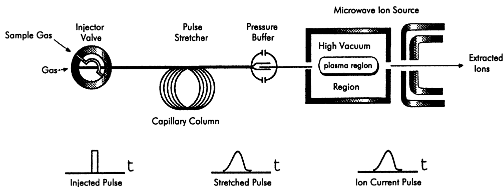
Fig. 3. Test device for loop injection into a microwave plasma ion source. One of two sample loops is shown; these inject samples into the carrier gas when the valve is rotated. The capillary column, 27 m of 0.32 mm silica capillary, is used to stretch out the pulse in time and the pressure buffer is an open split ( e.g. , Merritt et al. 1995), which removes pressure transients. The final capillary is 75 cm of 0.11 mm deactivated silica, as in Figure 1.
