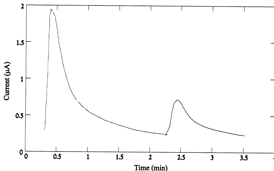
Fig. 4. Negative ^{12}\text{C} current pulses from 50 and 150 \mu\text{L} sample loops, injected 2 min apart. These pulses were recorded in a Faraday cup following magnetic analysis.
