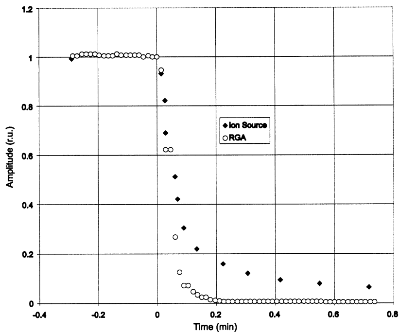
Fig. 5. Superposition of the tails of the ion pulse and gas pulse for mass 12. The gas pulse has a decay constant of 2.4 s, and the ion pulse is 3 s. Both pulses had a 4 min width.
