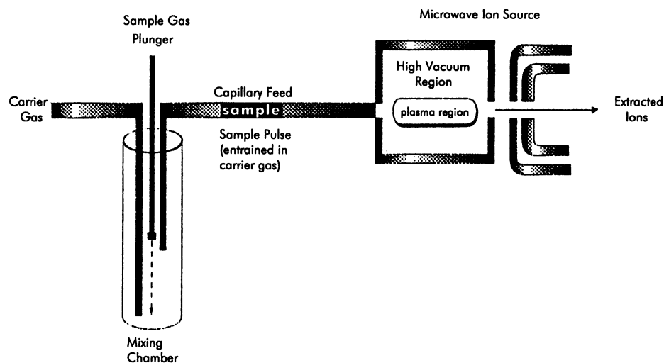
Fig. 1. Test device for injecting pulses of a sample gas into a carrier gas stream, and then into the microwave ion source. A continuous flow of carrier gas fills the mixing chamber, which is open to atmosphere at the top. When the plunger (a hypodermic needle) is depressed, the sample gas is mixed into the flow of carrier gas and is intercepted by the pickup capillary. Because this device is open, no pressure transient is introduced into the gas flow. Rectangular pulses of \text{CO}_2 are produced with a flow rate of ca. 0.2 \text{ mL min}^{-1} . A 75 cm length of 0.11 mm deactivated silica capillary leads to the ion source.
