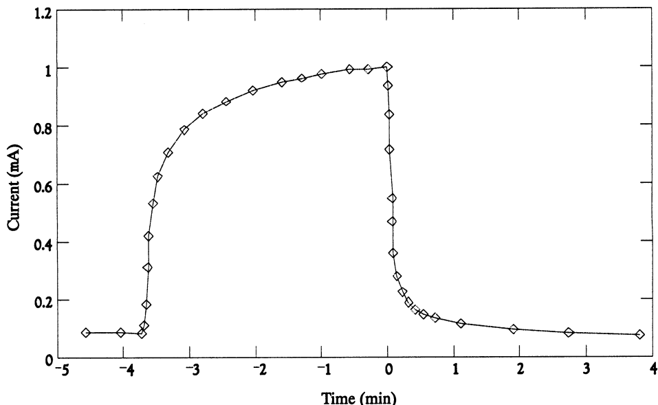
Fig. 2. A negative ^{12}\text{C} ion current pulse obtained from the microwave plasma ion source, followed by a charge exchange cell. Carbon dioxide was injected with the test pulse injector of Figure 1. The pulse duration was 4 min.
