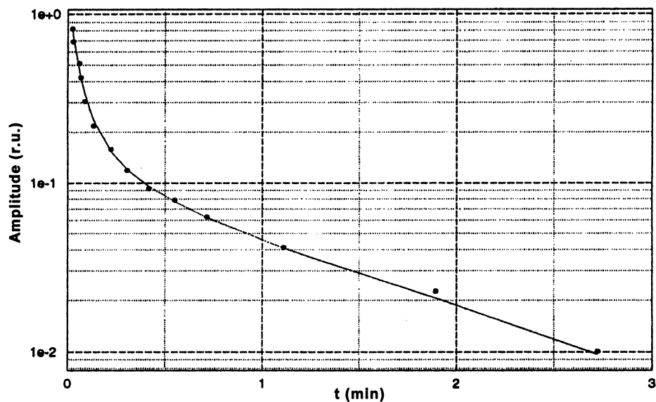
Fig. 6. Ion current tail, after turning off the gas pulse. The analyzed ^{12}\text{C} current decays initially with an exponential time constant of 3.06 s. The longer component is fitted well by a diffusion term having a diffusion coefficient of 0.684 \text{ cm}^2 \text{ min}^{-1} . The complete expression is f(t) = a + b \times \exp(-t/\tau) + c/(4\pi Dt)^{0.5} , where a = -0.0455 , b = 0.459 , c = 0.267 , \tau = 3.06 \text{ s} and D = 0.684 \text{ cm}^2 \text{ min}^{-1} .
