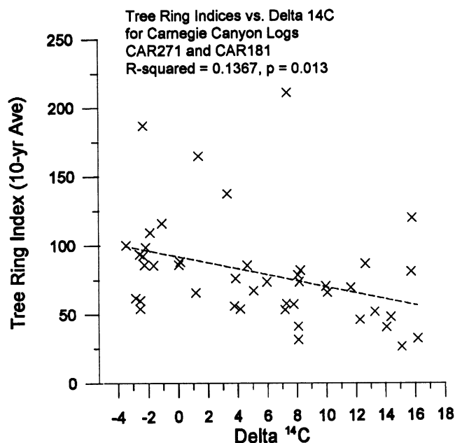
Fig. 2. Bivariate plot of \Delta^{14}\text{C} anomalies (file UWTEN93.14C [Stuiver and Reimer 1993]) with tree-ring indices for logs CAR271 and CAR 181 from Carnegie Canyon. The regression line (— —) demonstrates a negative correlation of ring indices and ^{14}\text{C} anomalies, i.e., positive anomalies are associated with reduced growth.
