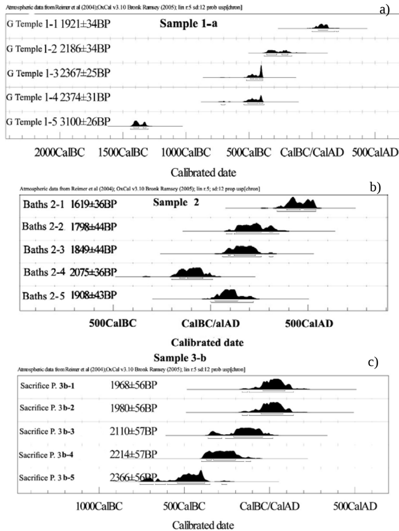
Figure 5 ^{14}\text{C} dates presented in multiple curves: a) sample 1; b) sample 2; c) sample 3
