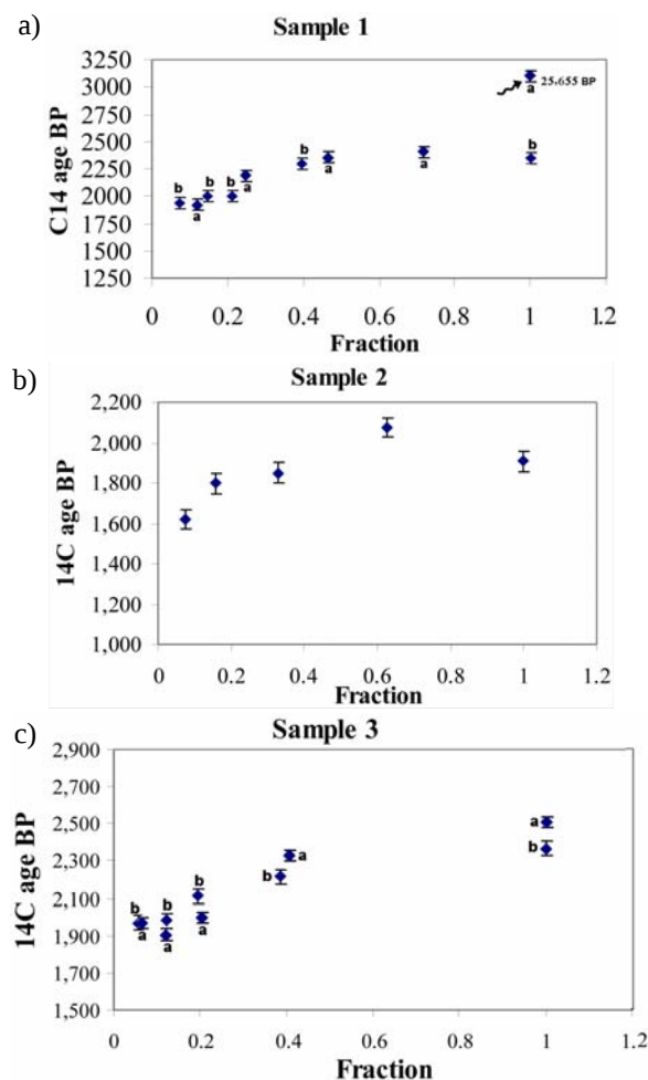
Figure 4 ^{14}\text{C} -F profiles: a) the 2 groups of determinations of sample 1 (a and b); b) sample 2; c) the 2 groups of determinations of sample 3 (a and b).
