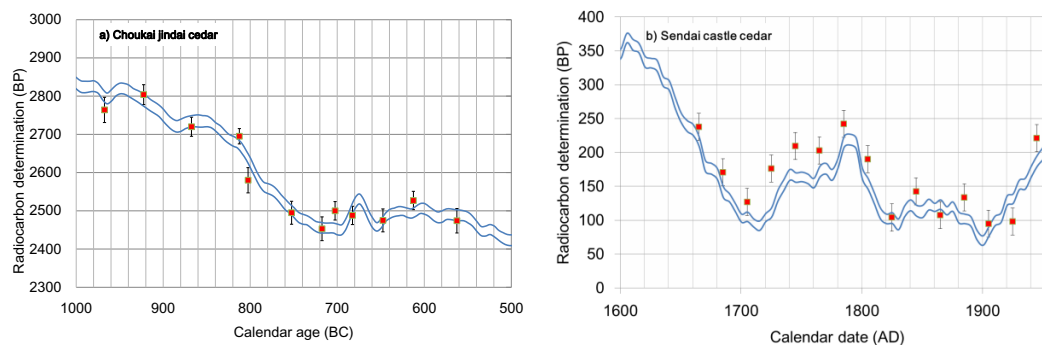
Figure 7 Comparison of ^{14}\text{C} concentrations of Tohoku-Japan trees with IntCal09 calibration curves. a) Choukai Jindai cedar in time range from BC 965 to 560 and b) Sendai castle cedar in time range from AD 1662 to 1965.
