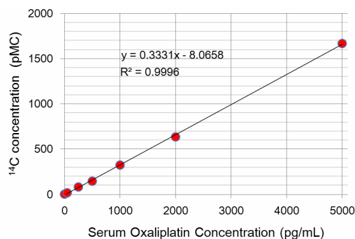
Figure 8 Relationship between concentration of ^{14}\text{C} -labeled oxaliplatin in serum and ^{14}\text{C} -concentration (pMC) obtained by AMS measurement.
