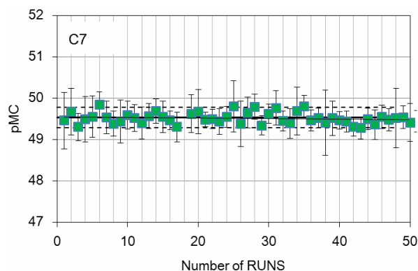
Figure 5 Long-term stability of YU-AMS system obtained over 20 months of ^{14}\text{C} concentration measurements for IAEA C7. Each solid line denotes the certified value of 49.54 pMC for IAEA C7. The dashed lines indicate an accuracy of 0.5% for the certified values.
