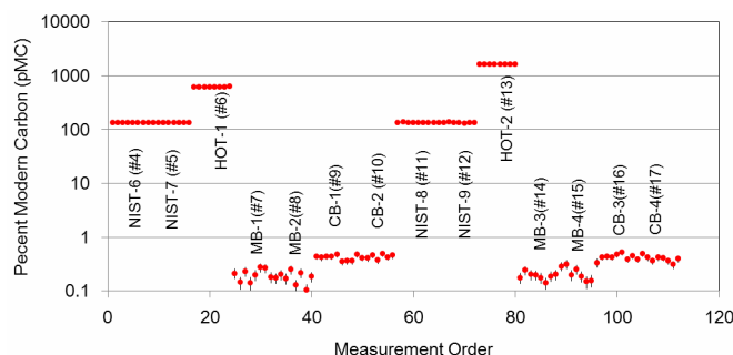
Figure 6 ^{14}\text{C} concentration (pMC) for 2 “hot” samples with F_m values of approximately 6 and 16. ^{14}\text{C} concentrations were indicated for the HOxII samples, and 2 each of machine background (MB) and chemical background (CB) samples before and after measuring each hot sample.
