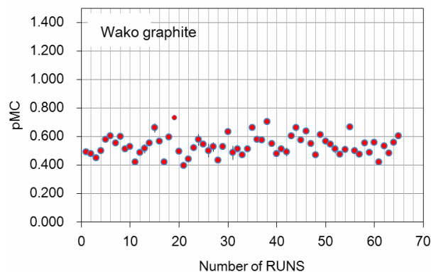
Figure 2 14 C concentration (pMC) of Wako graphite prepared with graphite preparation system over 2.5 yr of operation obtained with YU-AMS system.
