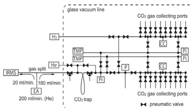
Figure 1 Schematic diagram of graphite preparation system employed in the YU-AMS. The system consists of an EA, an IRMS, and a \text{CO}_2 trapping system and can produce 20 graphite samples per day.
