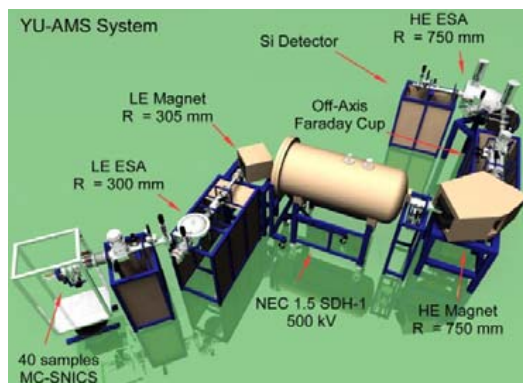
Figure 3 Schematic view of YU-AMS system. The ion source is placed at a 45° angle to allow possible future expansion with an additional ion source.
