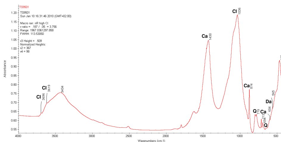
Figure 6 FTIR spectrum of sample TS9501: Cl = clay minerals; Q = quartz; Ca = calcite; Da = dahlite
