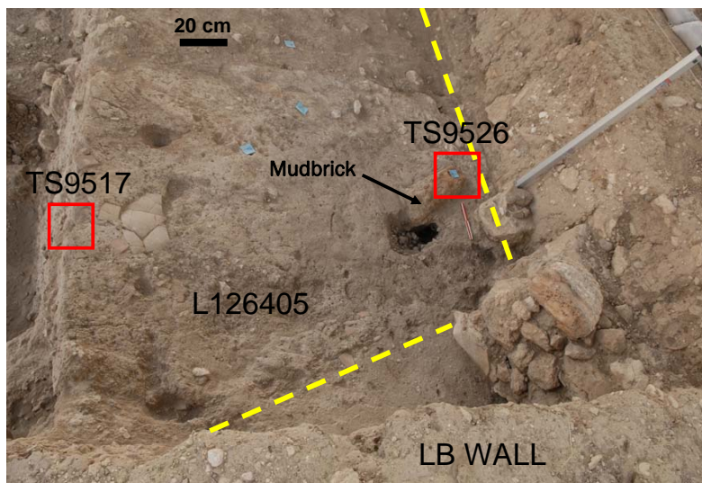
Figure 5 View from above of Locus 126405, Square 16C during the excavation, with the location of the blocks for micromorphology (squares). The dashed line marks the boundary of Locus 126405.
