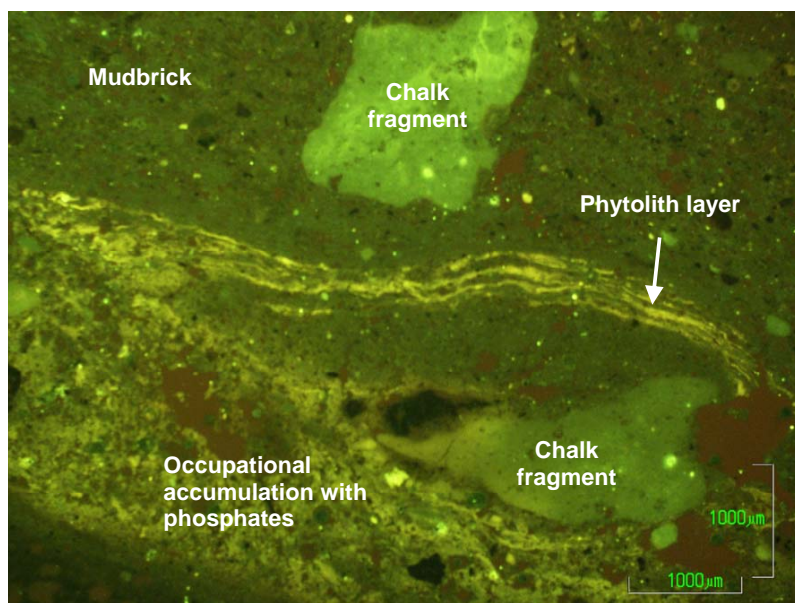
Figure 9 Microphotograph of sample TS9526, phytolith layer and associated occupational accumulation (BL, 2 \times ). Note the high autofluorescence (yellow hue) caused by the presence of phosphates.
