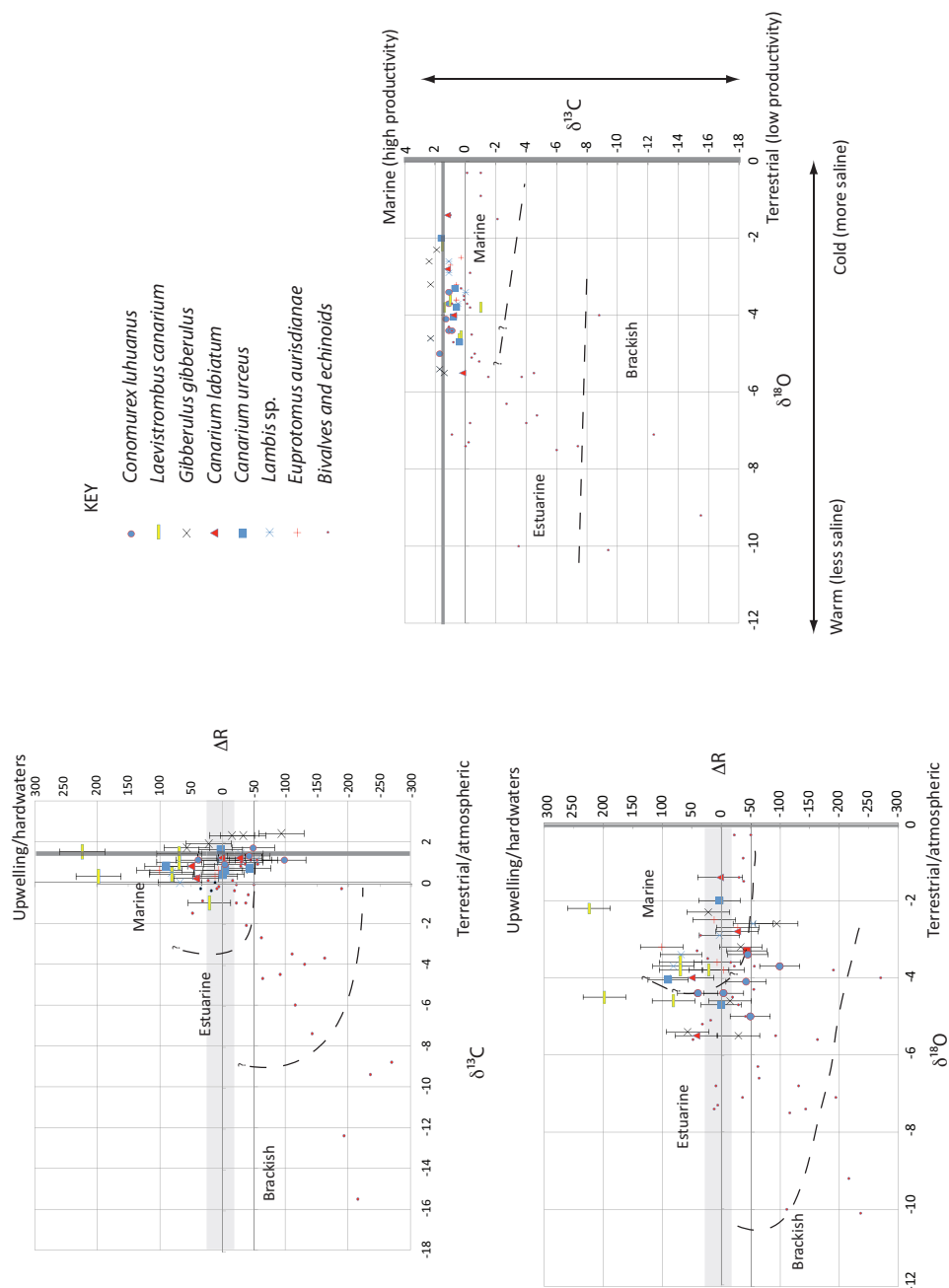
Figure 2 Measured \delta^{18}\text{O} , \Delta R , and \delta^{13}\text{C} values for Strombidae shells plotted against bivalve and echinoid isotopes (Petchey et al., in press) from Bogi 1, Caution Bay, southern PNG. At this location, the modeled \delta^{13}\text{C} isotopic composition of the modern surface ocean DIC is \sim 1.5\text{‰} and \delta^{18}\text{O} is \sim 0.3\text{‰} . The average \Delta R value for shellfish across the Pacific Gyre region is 6 \pm 21 \text{ } ^{14}\text{C yr} (see text for explanation). Average ocean isotope values ( \Delta R , \delta^{18}\text{O} , and \delta^{13}\text{C} ) are shown as gray bands. Dashed lines delineate approximate boundaries between the isotopic values for shells from different marine environments based on observations in the present study.
