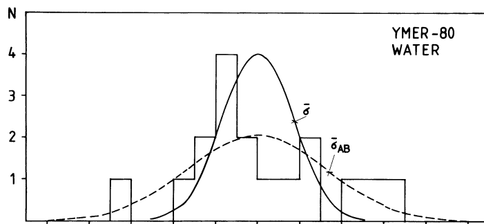
Fig 3. Distribution of the differences between the activities as measured with proportional counters 4 and 5 for 17 water samples. \sigma_{AB}/\sigma_{exp} = 1.88 .
