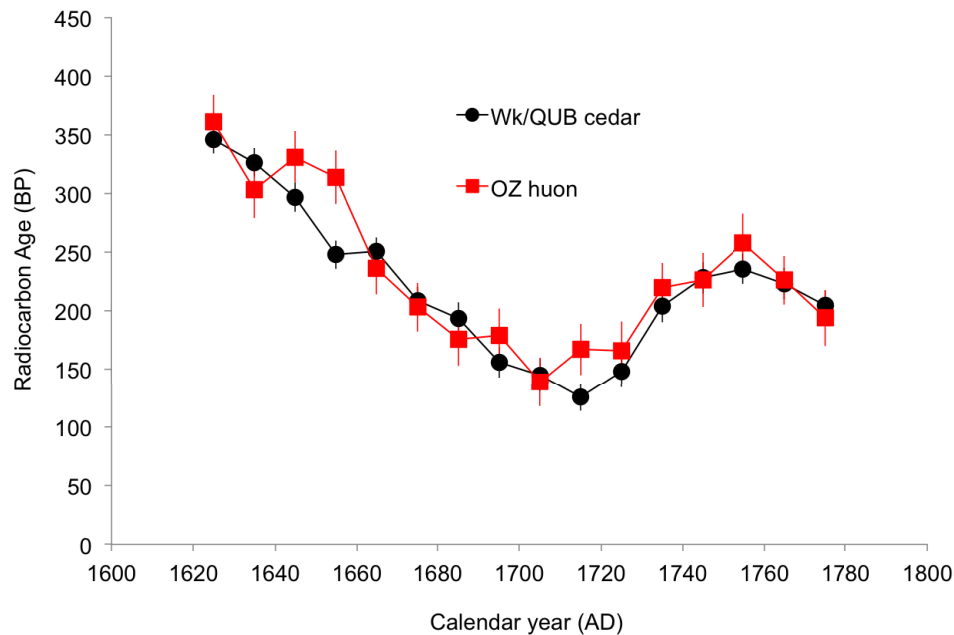
Figure 3 ^{14}\text{C} measurements ( 1\sigma errors) on decadal samples of dendrochronologically dated New Zealand cedar (mean Wk and QUB data; from Hogg et al. 2002) and Tasmanian huon pine (ANSTO - OZ huon data; from Hua et al. 2004) for the interval AD 1625 to 1775.
