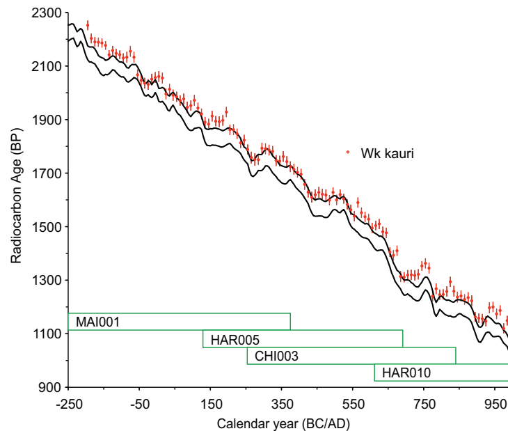
Figure 1 14 C measurements (1 \sigma errors) from dendrochronologically dated New Zealand kauri; overlain by the 95% probability envelope of IntCal09 (Reimer et al. 2009). The tree-ring periods covered by the 4 trees utilized in this study are also shown.
