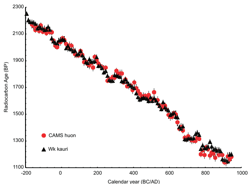
Figure 2 14 C measurements (1 \sigma errors) on decadal samples of dendrochronologically dated New Zealand kauri (Wk kauri) and Tasmanian huon pine (CAMS huon) for the interval 195 BC to AD 945.
