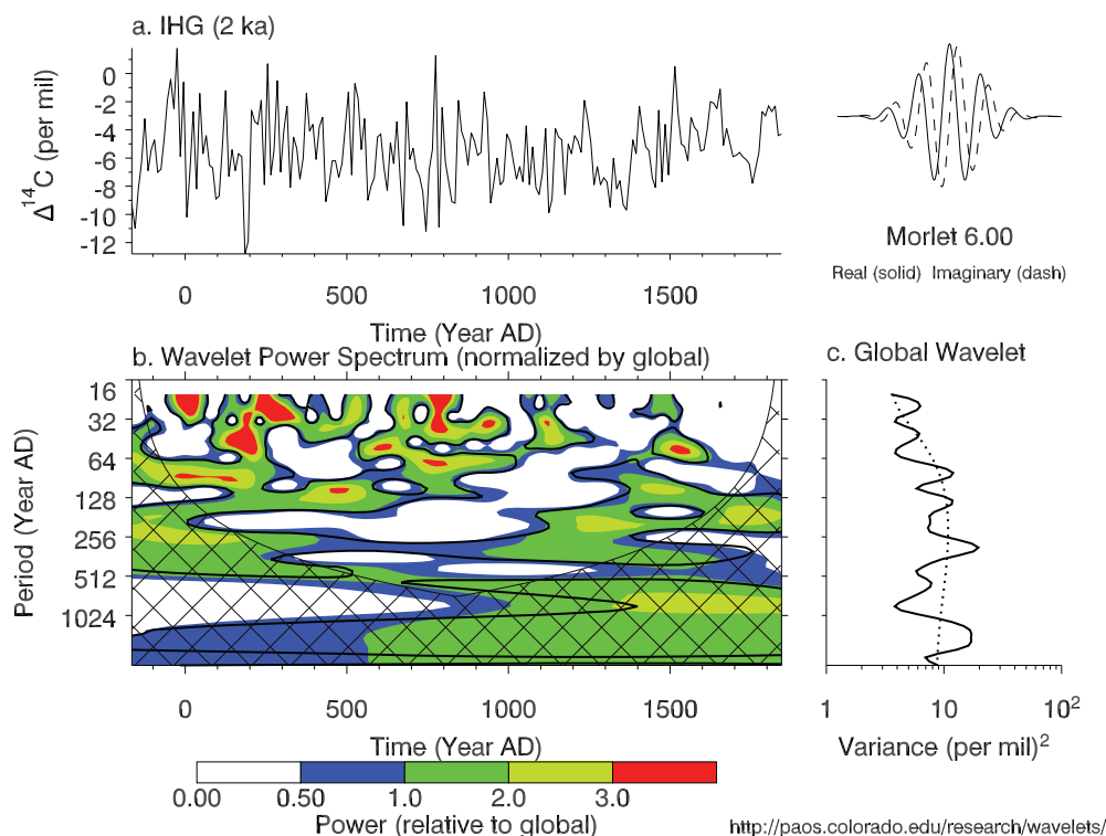
Figure 5 a) The interhemispheric gradient (IHG) for ^{14}\text{C} (SH-NH) from 200 BC to AD 1850. b) The wavelet power spectrum. The power has been scaled by the global wavelet spectrum (at right). The cross-hatched region is the cone of influence, where zero padding has reduced the variance. Black contour is the 90% significance level, using a red noise (autoregressive lag1) background spectrum. c) The global wavelet power spectrum (black line). The dashed line is the significance for the global wavelet spectrum, assuming the same significance level and background spectrum as in (b). See text for more details. Wavelet analysis after Torrence and Compo (1998).
