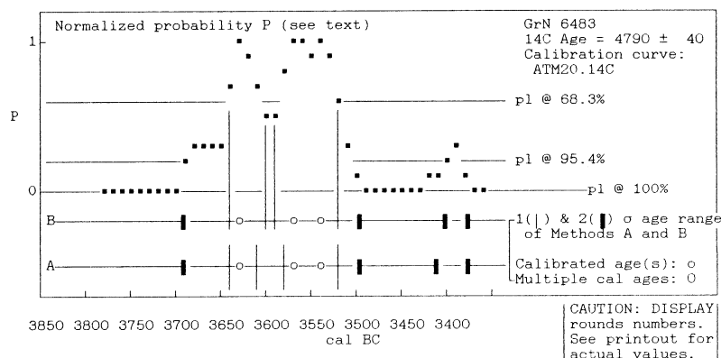
Fig 5. Graphic output for date A3 (Stuiver & Reimer)
