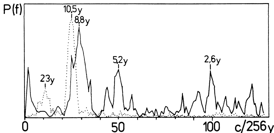
Fig 2. Power spectra from the \Delta^{14}\text{C} record (solid line) and sunspot record (dotted line). In order to avoid side lobes due to the length of the record, the spectra have been obtained by computing the amplitude of the sine wave best fitted to the data reduced to the first interval.
