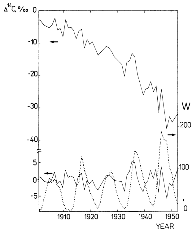
Fig 1. \Delta^{14}\text{C} record in tree-ring samples for the last century (upper curve); after corrections for the Suess effect (lower curve); sunspot record is shown for comparison (dotted curve)
