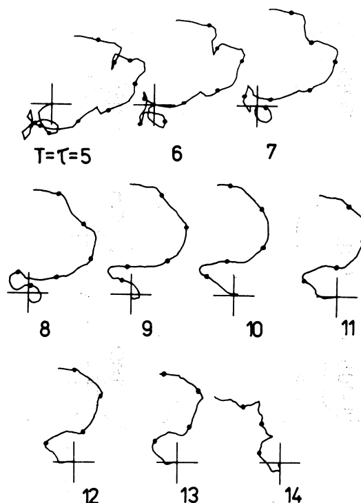
Fig 5. The cross-cyclogram analysis for T=\tau=5 - T=\tau=14 yr
