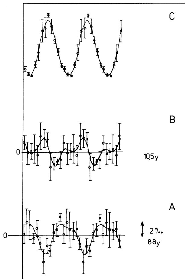
Fig 3. Input data reduction to the first interval: A. \Delta^{14}\text{C} with 8.8-yr interval; B. \Delta^{14}\text{C} with 10.5-yr interval; C. sunspots with 10.5-yr interval
