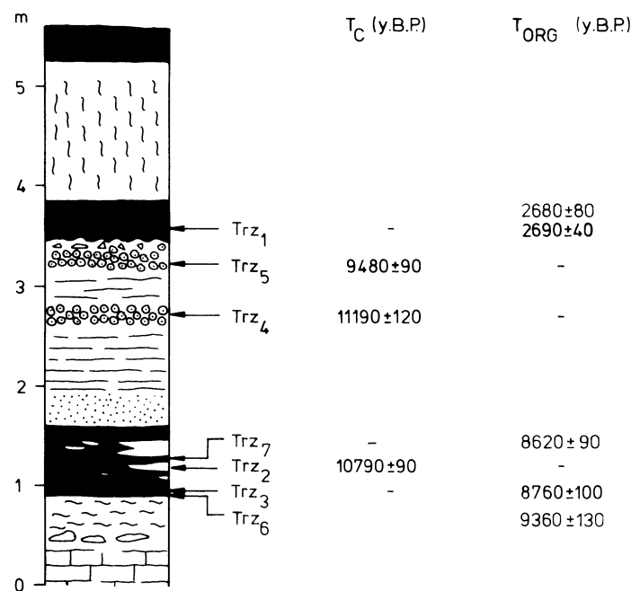
Fig 7. Cross-section through deposits of the Trzebienice site.
