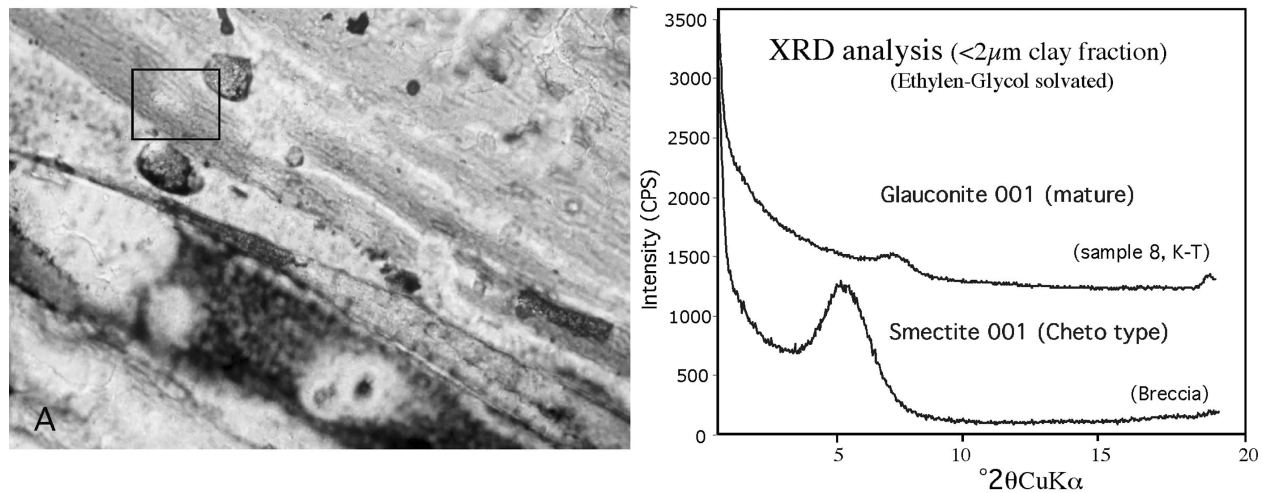
Fig. 4. Thin section micrograph of the green K/T clay layer (sample 8) with insert marking location of analysis. The XRD diffractogram of this green clay indicates the presence of mature glaucinite. In contrast, XRD analysis of breccia samples shows the presence of well-crystallized Cheto smectite, which is a typical alteration product of glass.
