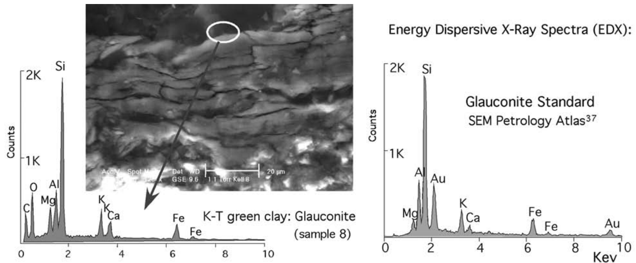
Fig. 5. Environmental SEM micrograph of the K/T green clay (sample 8) with electron diffractometer X-ray analysis that indicates a glaucinite composition. The glaucinite reference standard from the SEM petrology atlas (Welton 1984) is shown for comparison.
