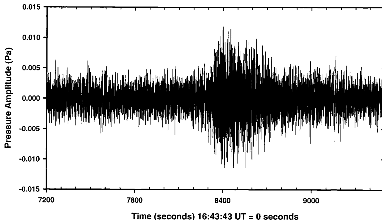
FIG. 4. Infrasonic signal produced by the Tagish Lake fireball as recorded at the IS10 Lac du Bonnet, Manitoba ( 50^\circ 12' \text{ N} , 96^\circ 1' \text{ W} ) infrasound station. The waveform has been bandpassed from 0.5 to 1.5 Hz. The range from IS10 to the terminal burst of the Tagish Lake fireball is 2640 km at a bearing of 309.2^\circ as seen from IS10. The signal arrives from an azimuth of 307^\circ .
