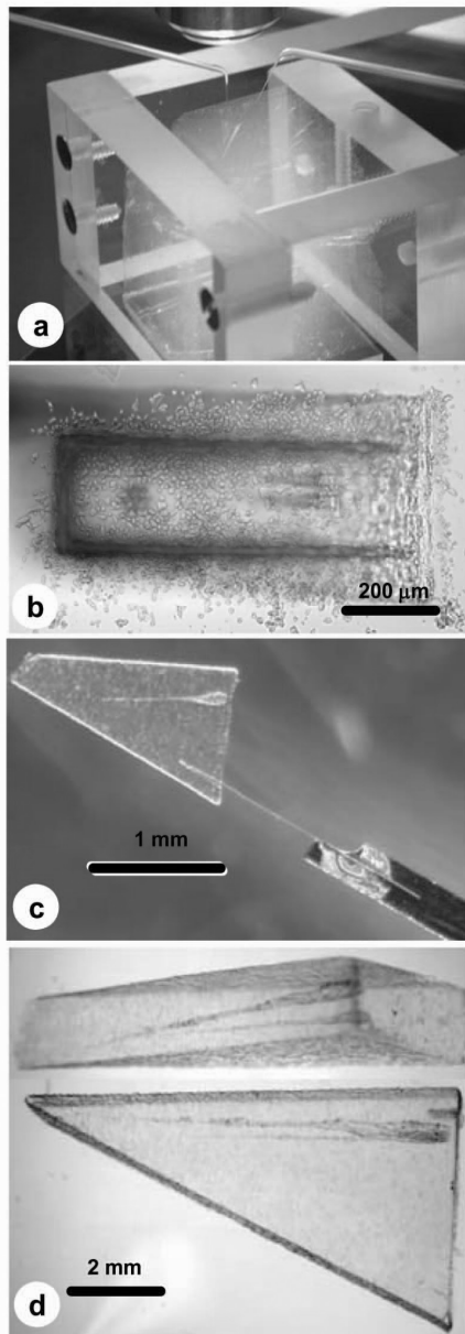
Fig. 5. The keystone system. a) Overview of the keystone system. An aerogel collector tile is fixed in a special vice and is viewed with a compound microscope. Two borosilicate glass microneedles (tip diameter \sim 1 \mu\text{m} , length \sim 1 \text{ cm} ) are attached to computer-controlled micromanipulators (not seen in this figure). A wedge-shaped white shadow in the aerogel is the “keystone.” b) Top view of a completed keystone before removal from the aerogel collector tile. A clamp-shaped groove is the side cut, and the light contrast vertical line is the entrance of the undercut. A dark round shadow in the middle left inside the keystone is the cometary feature (track #94). Two horizontal lines are holes for supporting the microforklift. This aerogel tile C2078 was found to be especially hard, and generated quite an amount of aerogel debris during the operation. c) A keystone fixed on a microforklift, including a cometary track 104 (1 mm long bulb + stylus). d) The biggest keystone generated at the JSC Stardust curation facility, viewed from two different directions. This 8.5 mm long keystone includes two spiral carrot cometary tracks #99 (7 mm long; thinner track in this figure) and #100 (8 mm long).
