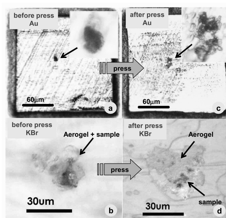
Fig. 8. Preparation of a cometary grain for spectroscopy. a) A cometary particle (C2054, 0,35,91,0) set on a Au mount. b) A cometary particle (C2054,0,35,87,0) set on a KBr mount. c) After pressing of the sample in (a). Note that the Au mount surface as well as the sample are flattened. d) After pressing of the sample in (b).
