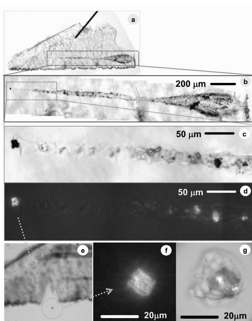
Fig. 7. A series of images acquired following the extraction of a keystone including the cometary track 48 (from aerogel tile C2027, 2117 \mu\text{m} long track). a) A photo mosaic of the entire keystone on a microforklift composed by three pictures taken under transmitted light by a Nikon compound microscope with a 10 \times objective lens. b) A higher magnification mosaic image of track 48 showing more details of the feature. 13 individual images were taken under both transmitted and reflected lights using a 20 \times objective lens with different focusing, and compressed as a 3-D image using computer photo processing. c) A bright-field view of the boxed area of track 48 in (b) including the terminal particle in with transmitted/reflected combined lights. d) A dark-field view of the same area with (c) in a reflected cross-polarized light. e) A captured image from a movie taken by a CCD camera attached to the stereomicroscope, right after the particle was removed from the keystone. f) A dark-field image of the extracted terminal particle of track 48. g) A bright-field image of the extracted terminal particle.
