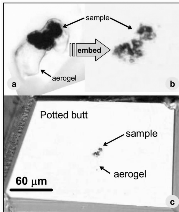
Fig. 9. Embedding cometary grains. a) A Wild 2 cometary grain #16 extracted from track 35 (from C2054 aerogel tile, C2054,0,35,16,0). This grain is surrounded by compressed aerogel observed in the lower and right side of the grain. b) The same grain of (a) after embedded in low-viscosity Embed 812 epoxy and sliced using an ultramicrotome. The compressed aerogel is almost invisible in the epoxy. The shape of the grain is well preserved. c) The potted butt of the grain. The ultramicrotomed thin sections from this potted butt are shown in Fig. 11.
