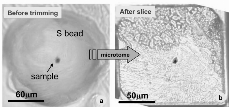
Fig. 10. Embedding a cometary grain in beaded sulfur. a) A pure sulfur potted butt of a Wild 2 cometary grain #1 (the terminal particle) of track 17. The pure sulfur embedding medium is crystalline, nearly transparent, dome shape attached to an epoxy base. b) The same sample after slicing by ultramicrotome. Sulfur vaporizes immediately, making a patchy structure.
