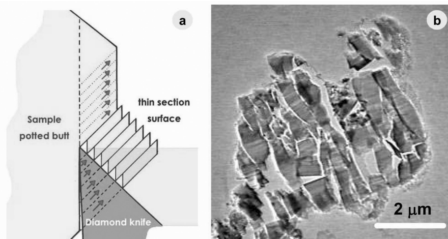
Fig. 12. Ultramicrotomy-induced damage (chattering). a) Schematic image of structural damage caused by the diamond knife. Adapted and modified after Reid (1975). b) A bright-field TEM image of an ultramicrotomed thin section of a Wild 2 cometary particle (C2027, 3,32,3,2), one of the terminal particles from so-called twin tracks 32 and 69.
