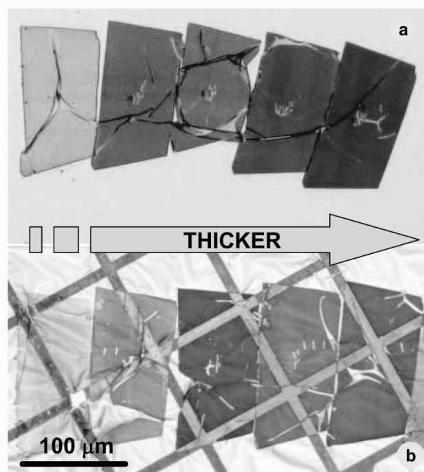
Fig. 11. Ultramicrotomed sections. a) Ultramicrotomed thin sections mounted on a silicon wafer substrate. b) Ultramicrotomed thin sections mounted on an amorphous carbon film supported Cu TEM grid. These slices are from the same potted butt grain sample shown in Fig. 9. The sections show color differences due to varying thicknesses. In (a), the thin section at the far left is 50 nm thick and 100 nm thick at the far right. In (b), the far left thin section is 40 nm in thickness, and the reddish thin section (far right) is 150 nm thick.
