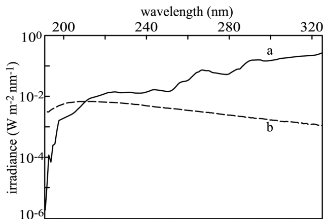
Fig. 4. a) A comparative chart of the irradiance of the surface noon lighting at the equator of Mars (from Patel et al. 2002). b) The light delivered at the working distance of 145 mm from the discharge region of the deuterium lamp.
