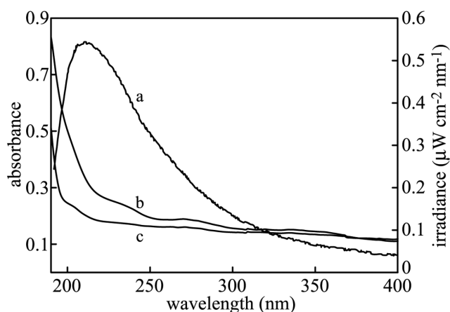
Fig. 7. a) The spectrum of the deuterium lamp between 190–400 nm, recorded at the same distance from the lamp as the amino acid film, scaled to the right ordinate. The UV-visible absorption spectra of a \sim 300 nm layer of (b) solid glycine and (c) solid D-alanine on a silicon disc, in the range 190–400 nm, scaled to the left ordinate.
