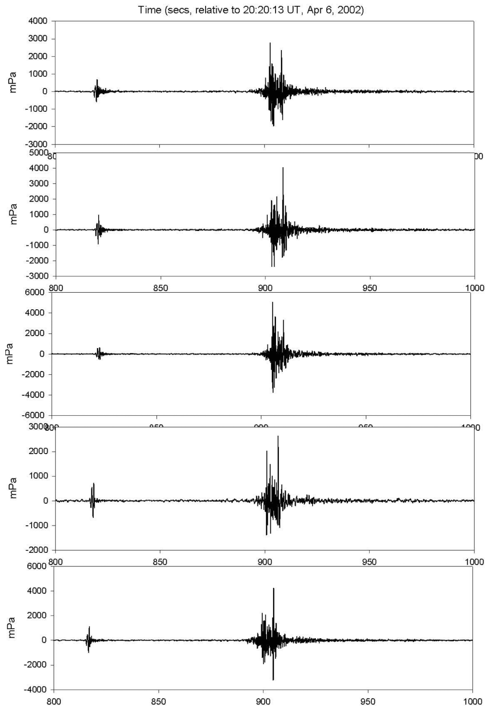
Fig. 9. The recorded infrasound signal on all five channels at Freyung for the Neuschwanstein fireball. Note that these waveforms have been high-passed above 0.40 Hz to most clearly define the fireball signal. The time is relative to 20:20:13 UT on April 6, 2002.
