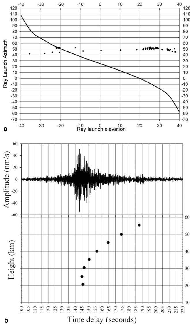
Fig. 15. a) The azimuth at which modeled rays were launched from the source (along the fireball path) as a function of the modeled ray launch elevation (relative to the horizontal at 0°). Each point represents one ray that is able to reach Freyung from a point along the fireball path. The bold line represents those points that are at right angles to the fireball trajectory; b) the vertical seismic component for station SQTa (top) showing airwave arrival near a time delay of 145 sec. The bottom plot shows the modeled time delays from point sources distributed along the fireball trajectory (as a function of height).
