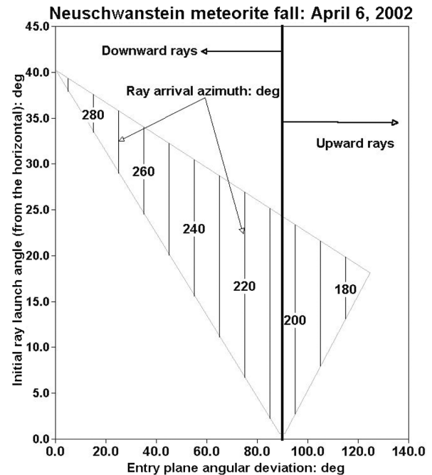
Fig. 16. Initial ray launch angle from the horizontal (°) versus the line source entry plane deviation (°) for Neuschwanstein.
