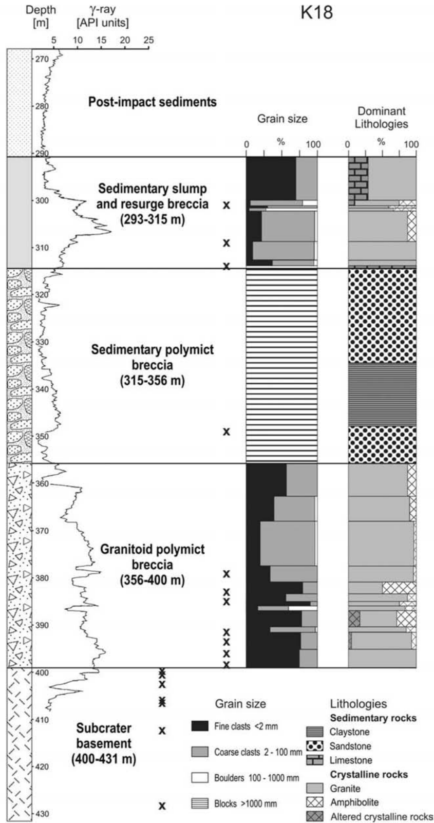
Fig. 4c. Lithological log of the drill core, grain size distribution, and lithological composition of allochthonous breccias from the crater interior in borehole K18. Visual logs with \gamma -ray graphs are given in American Petroleum Institute (API) units (normalized for counts per second). The lithological composition is based on visual counting and the \gamma -ray log. "x" marks the positions of samples taken for geochemical analyses.
