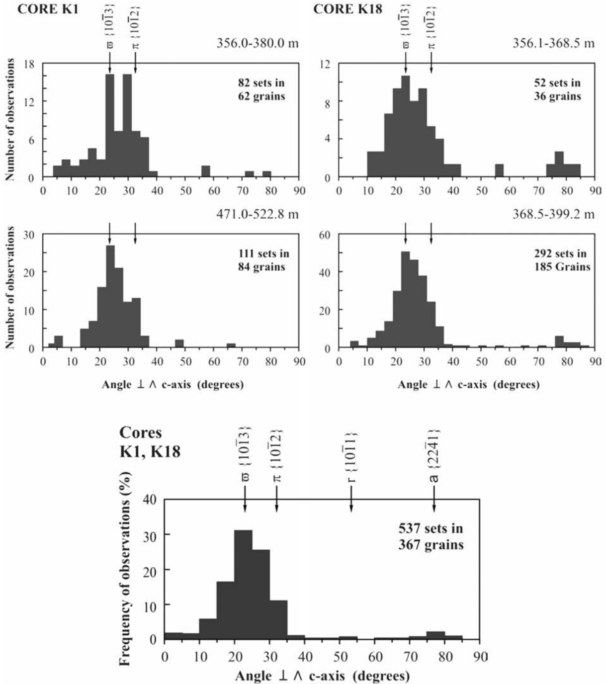
Fig. 5. Distribution of PDF orientations in quartz of granite-derived polymict breccia samples from cores K1 and K18. Top: histograms showing the number of PDF planes in 3^\circ binning versus the angle between the c-axis and PDFs. Bottom: histogram combining all sets from the top with 5^\circ binning.
